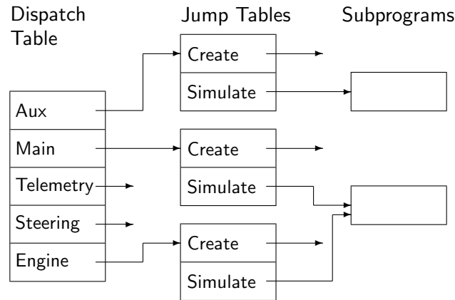
Figure 6.6: Implementation of dynamic dispatching
