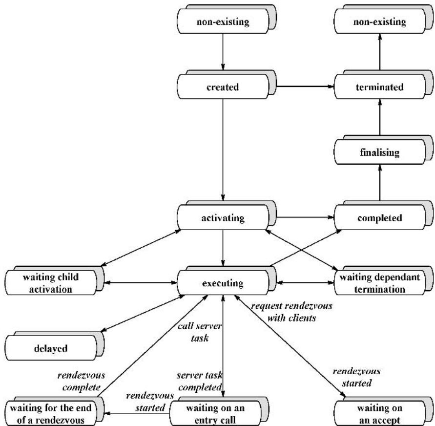
Fig. 5.2: Summary of task states and state transitions
