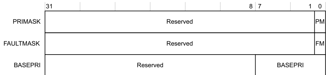
Figure B1-2 The special-purpose mask registers
