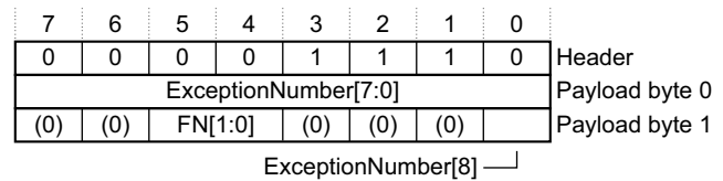
Figure D4-15 Exception trace packet format
