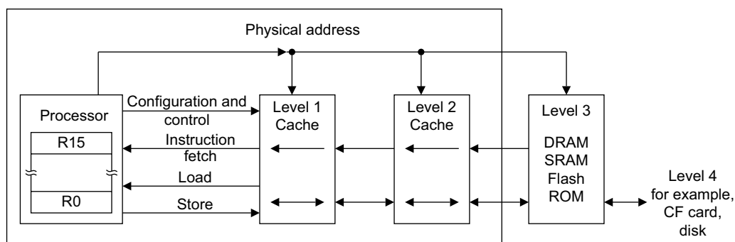
Figure A3-9 Multiple levels of cache in a memory hierarchy
