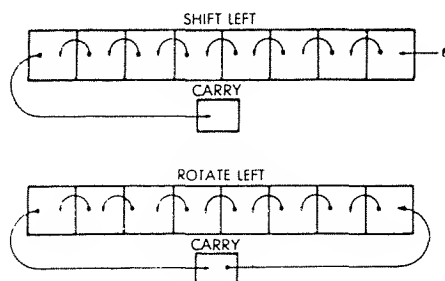
Fig. 4.9: Shift and Rotate
