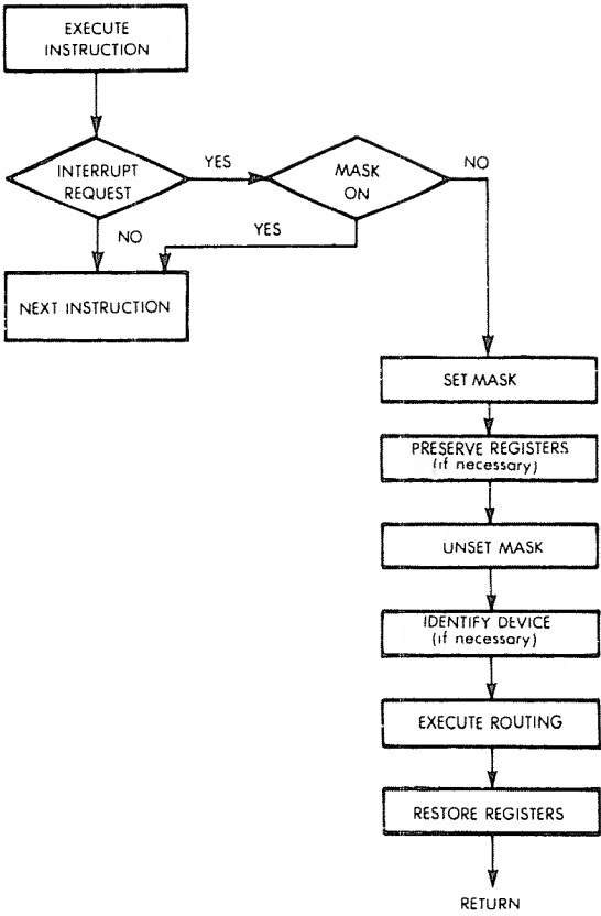
Fig. 6.34: Interrupt Logic
