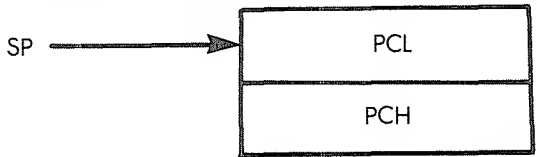
Fig. 6.22: Z80 Stack After Interruption
