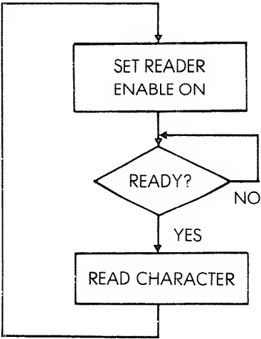
Fig. 6.20: Reading from a Paper-Tape Reader
