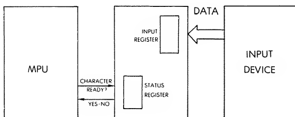
Fig. 6.8a: Handshaking (Input)
