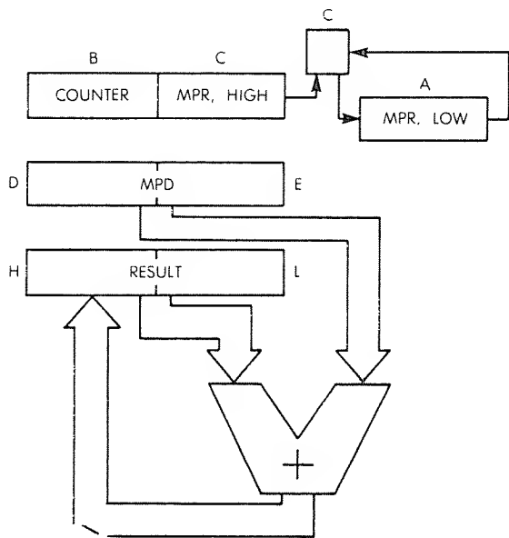
Fig. 3.27: 16 × 16 Multiply—The Registers
