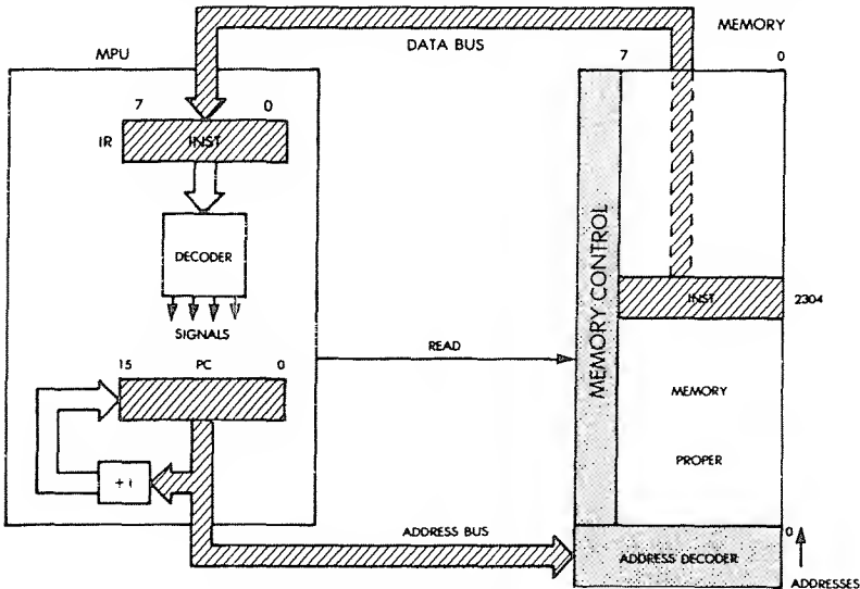
Fig. 2.7: Automatic Sequencing
