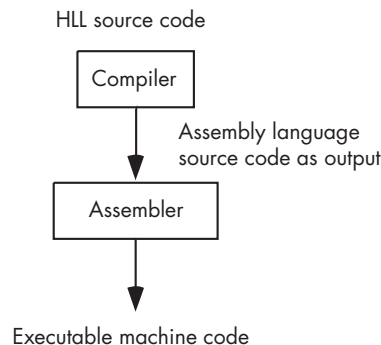
Figure 5-8: Emission of assembly code by a compiler
