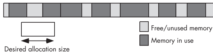
Figure 11-3: Memory fragmentation
