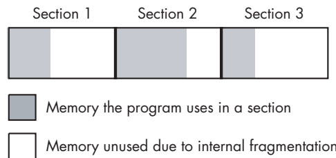
Figure 5-11: Internal fragmentation
