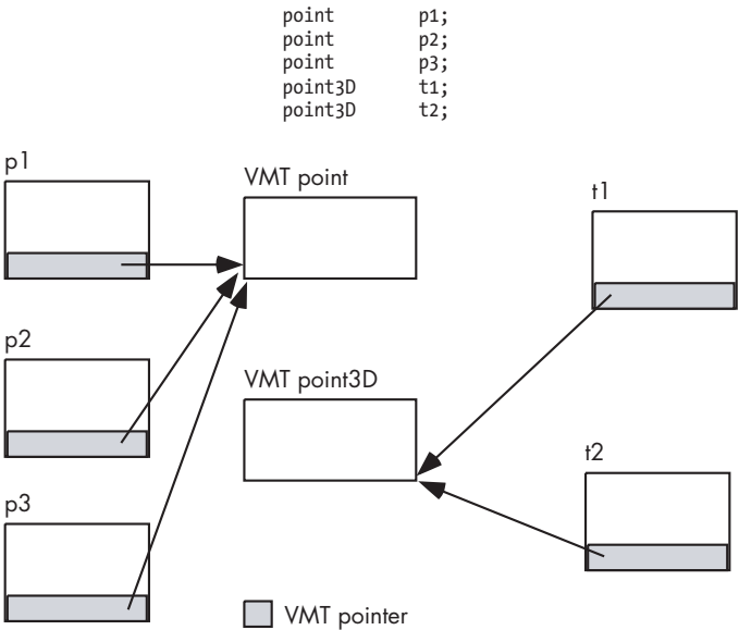
Figure 12-9: Virtual method table access
