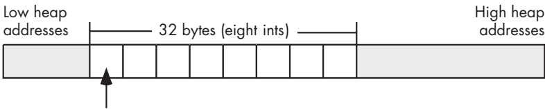
Pointer (address) that malloc( sizeof( int ) * 8 ) returns
