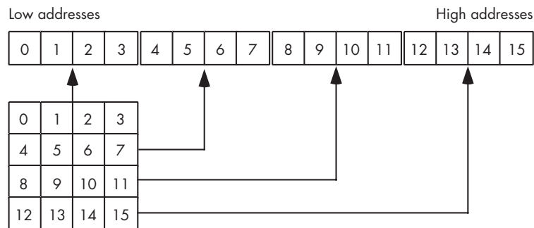
Figure 9-5: Another view of row-major ordering for a 4×4 array
