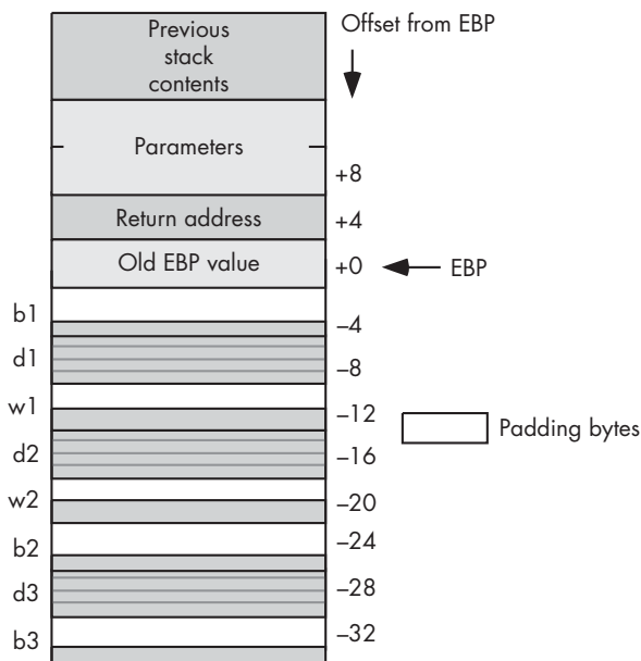
Figure 8-12: RISC compilers force aligned access by adding padding bytes
