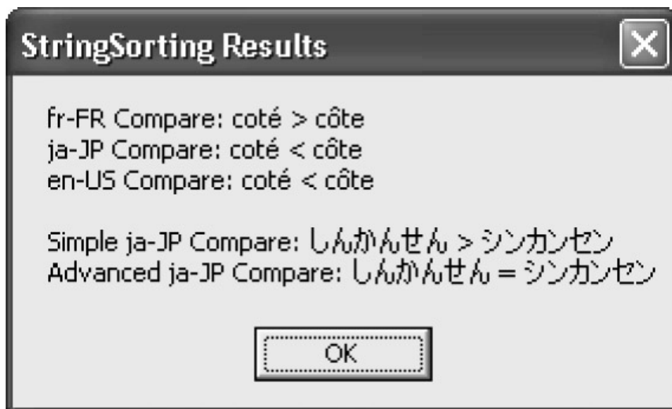
Figure 12–1: StringSorting results
