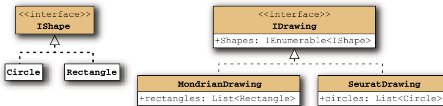
Figure 3.4 Interfaces for shapes and drawings, and two implementations of each
