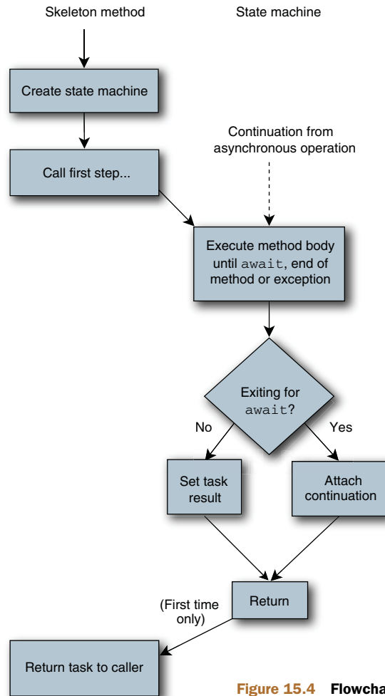
Figure 15.4 Flowchart of generated code
