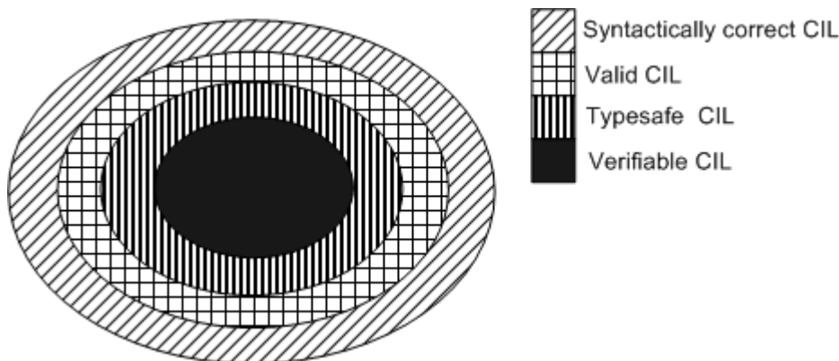
Figure 1: Relationship between correct and verifiable CIL
