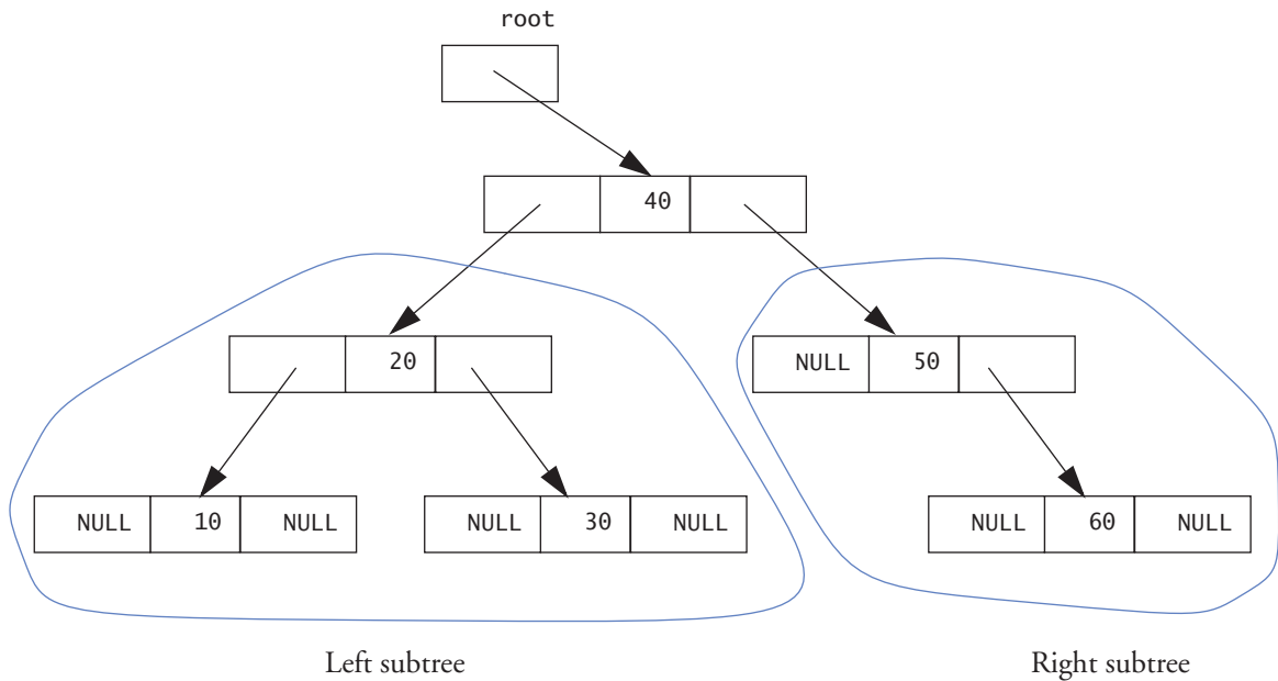
Display 17.23 A Binary Tree
