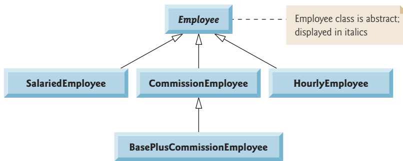
Fig. 13.11 | Employee hierarchy UML class diagram.
