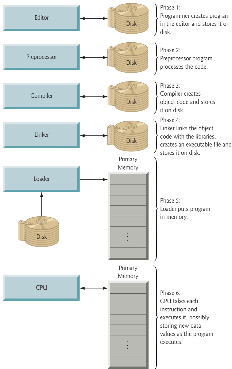
Fig. 1.1 | Typical C++ environment.
