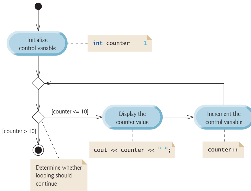
Fig. 5.4 | UML activity diagram for the for statement in Fig. 5.2.
