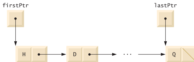
Fig. 20.2 | A graphical representation of a list.
