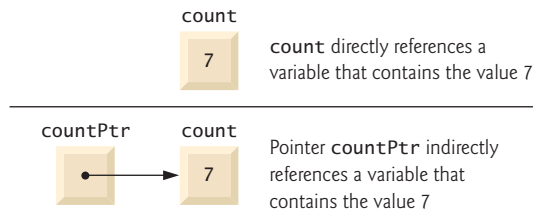
Fig. 8.1 | Directly and indirectly referencing a variable.
