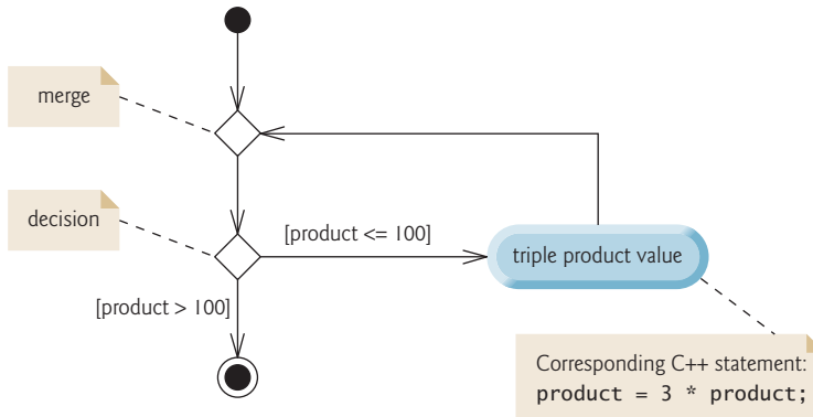
Fig. 4.6 | while repetition statement UML activity diagram.
