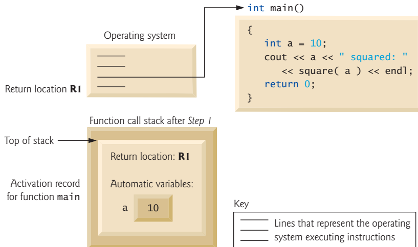
Fig. 6.14 | Function call stack after the operating system invokes main to execute the program.
