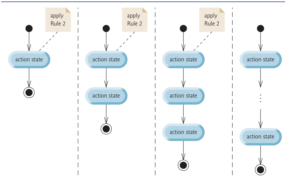
Fig. 5.23 | Repeatedly applying Rule 2 of Fig. 5.21 to the simplest activity diagram.
