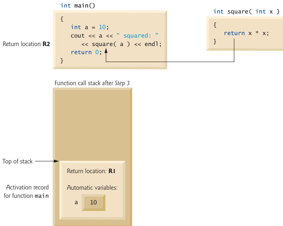
Fig. 6.16 | Function call stack after function square returns to main .
