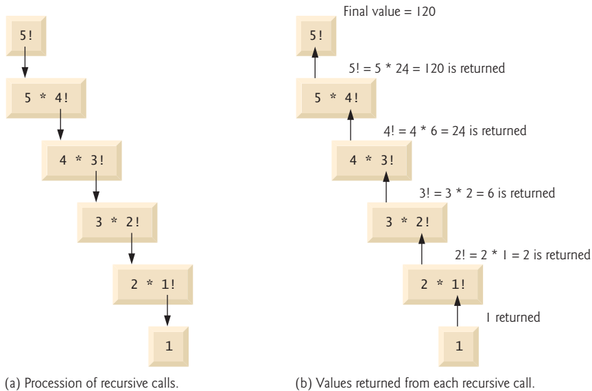
Fig. 6.28 | Recursive evaluation of 5!.
