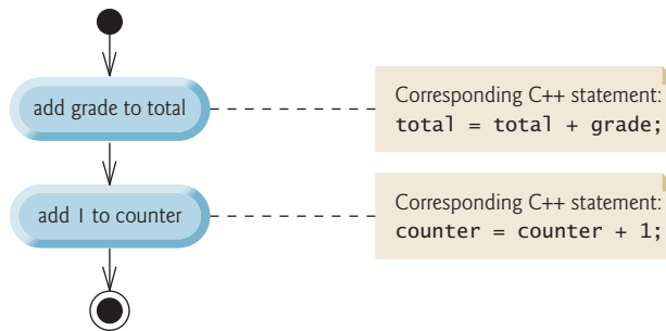
Fig. 4.2 | Sequence-structure activity diagram.
