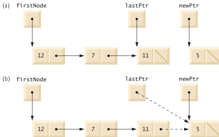
Fig. 20.7 | Operation insertAtBack represented graphically.
