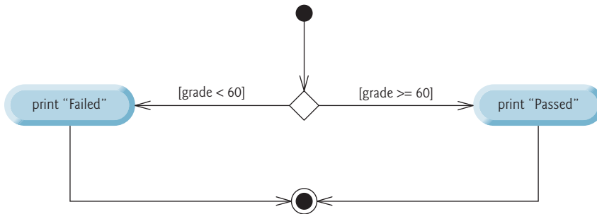
Fig. 4.5 | if...else double-selection statement activity diagram.
