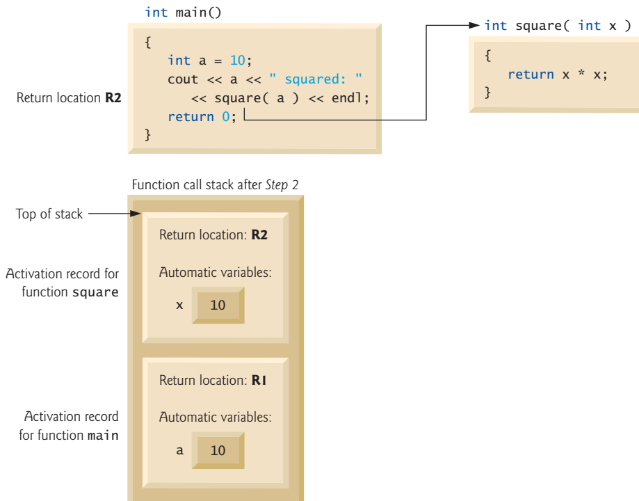
Fig. 6.15 | Function call stack after main invokes square to perform the calculation.
