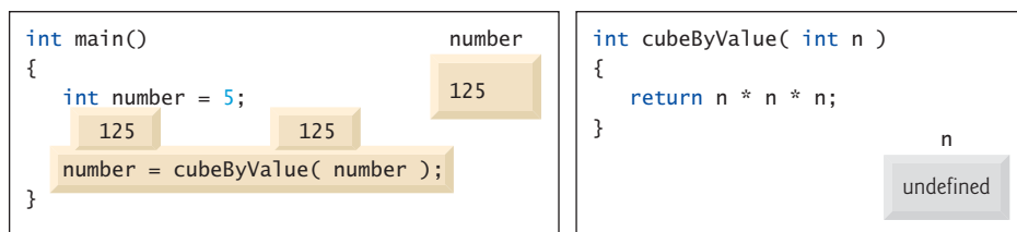
Fig. 8.8 | Pass-by-value analysis of the program of Fig. 8.6.
