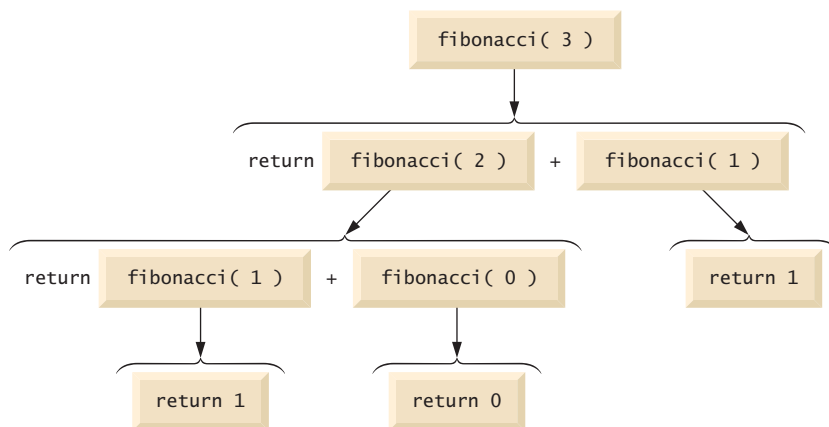
Fig. 6.31 | Set of recursive calls to function fibonacci .
