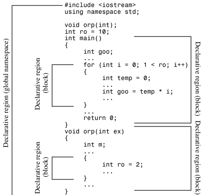
Figure 9.5 Declarative regions.
