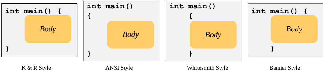
Figure 4.3 The most common C++ coding styles.
