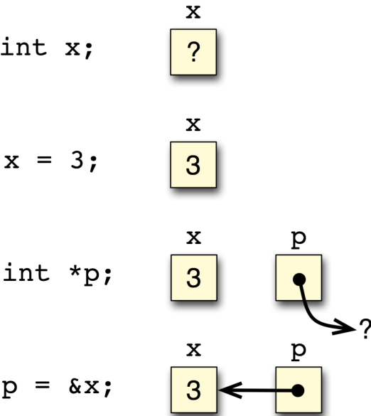
Figure 10.2 Pointer declaration and assignment
