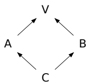
Figure 4 — Virtual base
