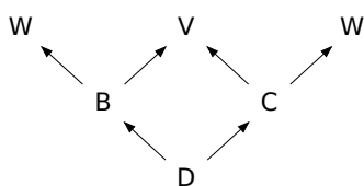
Figure 6 — Name lookup
