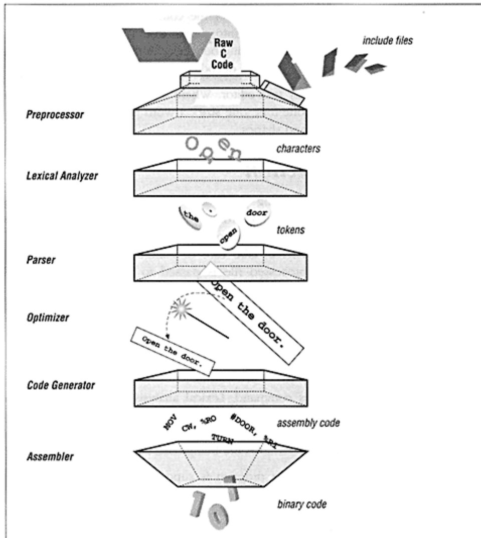
Figure 23-3 Compiler modules
