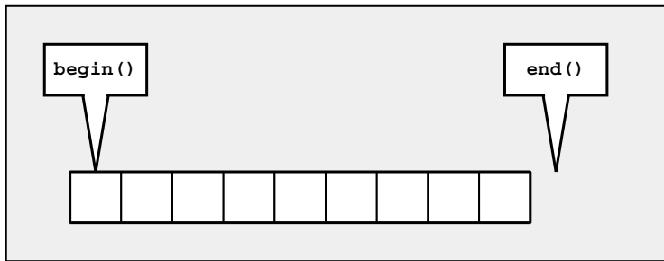
Figure 6.4. begin() and end() for Containers
