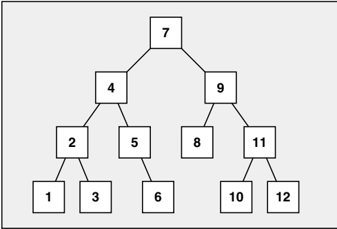
Figure 7.13. Internal Structure of Sets and Multisets
