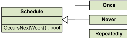
Figure 5.2 Representation of schedule using the usual object-oriented design with functionality implemented using virtual methods.
