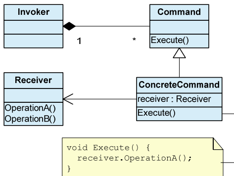
Figure 8.2 'Invoker' stores a collection of classes implementing the 'Command' interface. When invoked,
