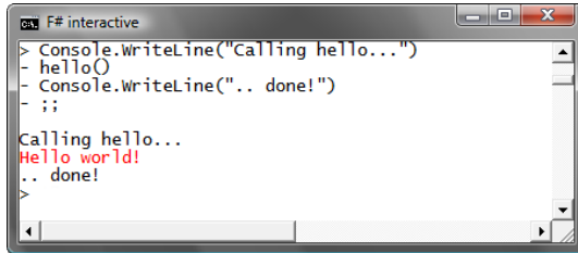
Figure 9.2 Changing the color of the console text using 'changeColor' function. You can see that the color is changed only inside the 'hello' function and then the original color is restored.
