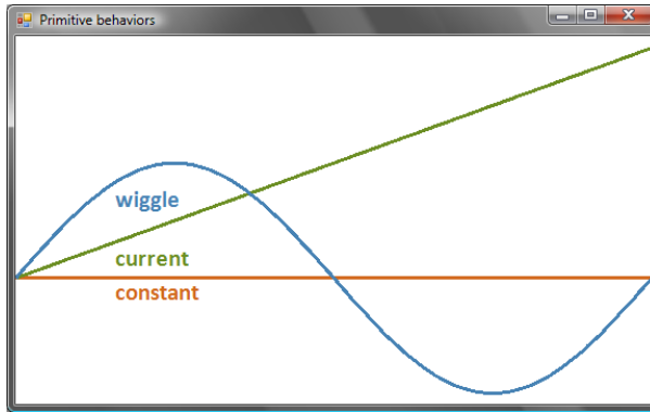
Figure 15.2 Primitive behaviors during the first two seconds. The value of 'current' ranges from 0 to 2 and 'wiggle' oscillates between +1 and -1.
