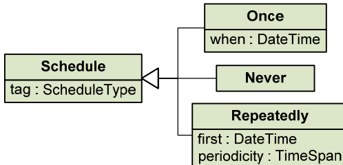
Figure 5.1 Class hierarchy for representing three different types of schedule with different properties for every case.
