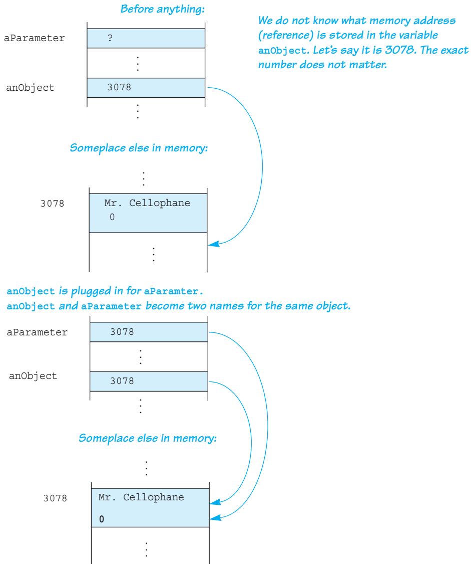
Display 5.15 Memory Picture for Display 5.14 (part 1 of 2)
