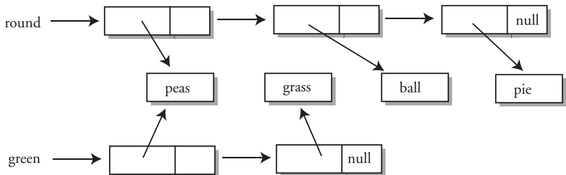
Display 15.36 Sets Using Linked Lists
