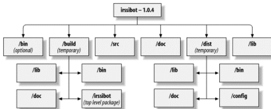
Figure 3-1. irssibot directory structure
