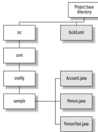
Figure 1-1. Starting point for our example buildfile
