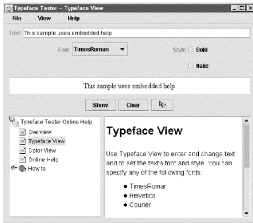
Figure 7.8. Embedded help
