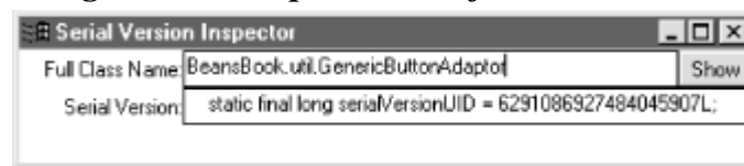
Figure 5.6. Graphical interface to serialver
