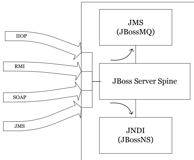
Figure 4: Detached invokers
