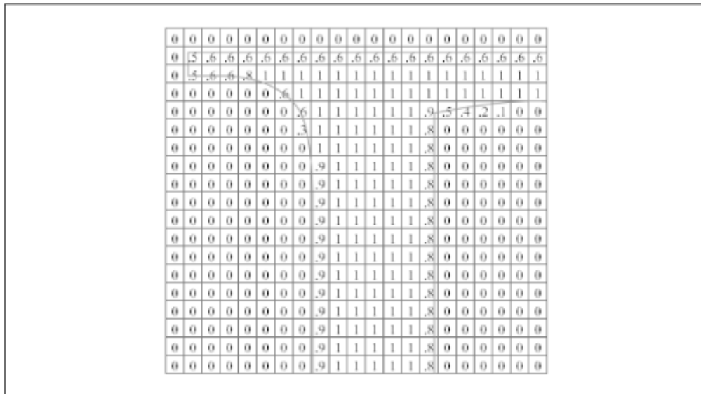
Figure 2.5. The rasterizer produces an alpha value for every pixel
