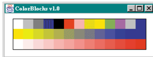
Figure 15.8. ColorBlocks output
