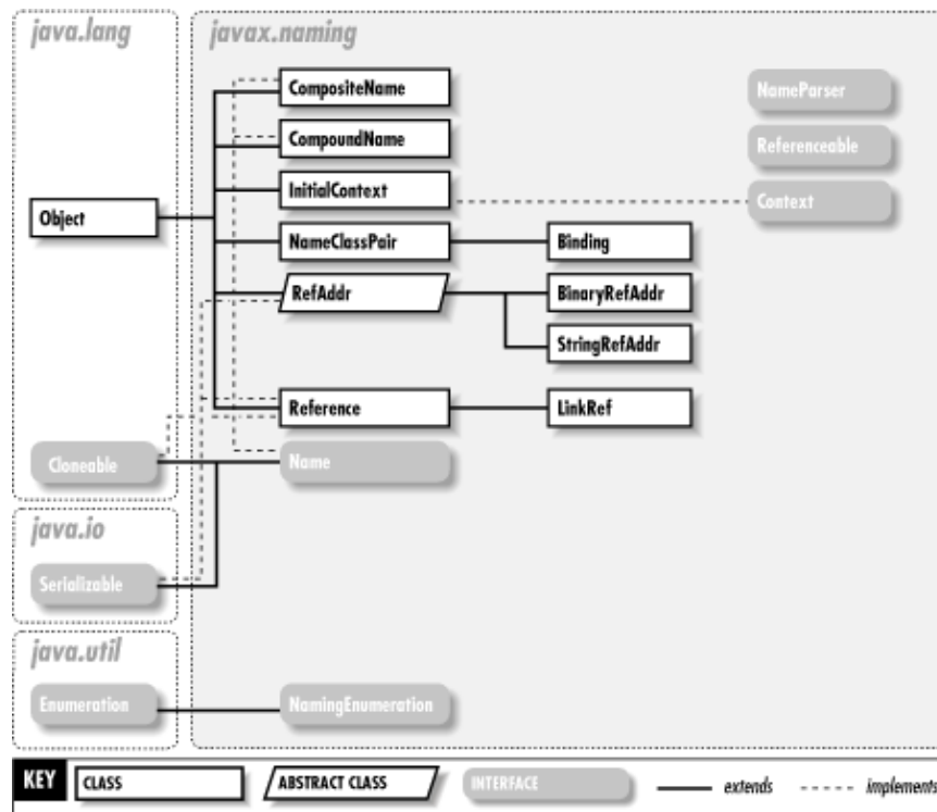
Figure 22-1. The classes and interfaces of the javax.naming package
