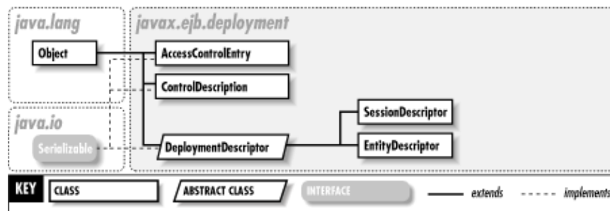
Figure 20–1. The javax.ejb.deployment package class hierarchy
