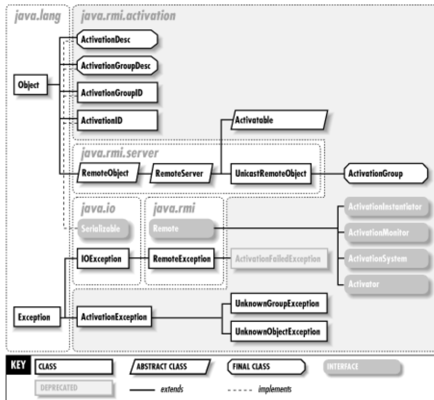
Figure 14–1. The java.rmi.activation package
