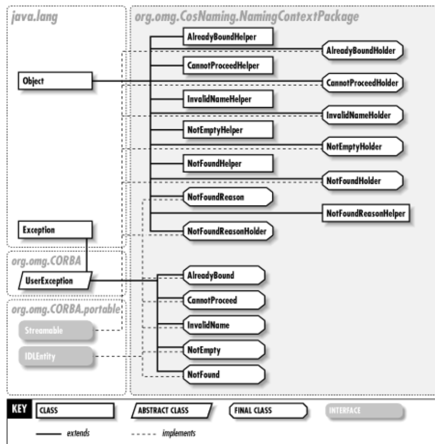
Figure 36–1. The org.omg.CosNaming.NamingContextPackage package
