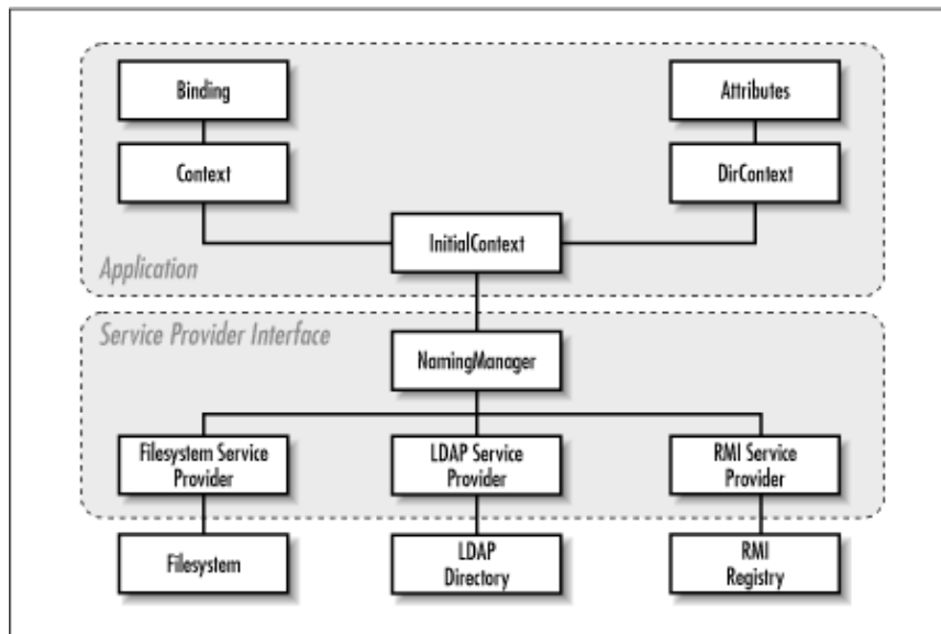
Figure 6-1. The JNDI architecture
