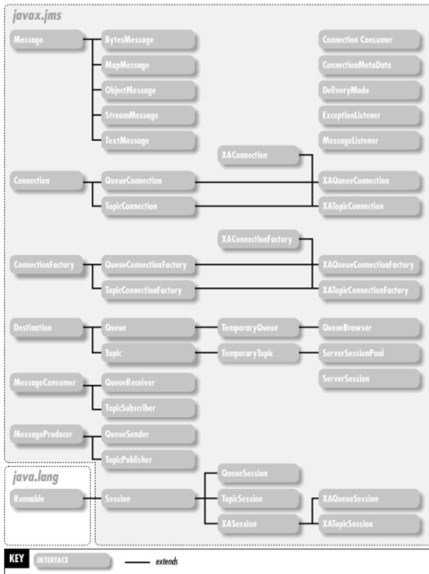
Figure 21–1. The interfaces of the javax.jms package
