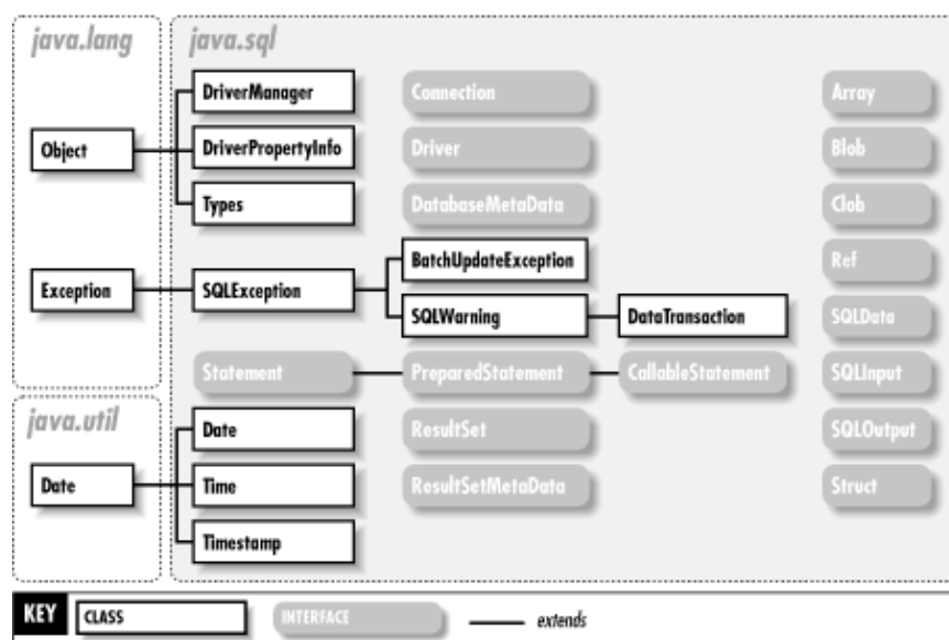
Figure 18–1. The java.sql Package
