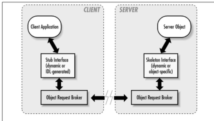
Figure 4-1. Basic CORBA architecture
