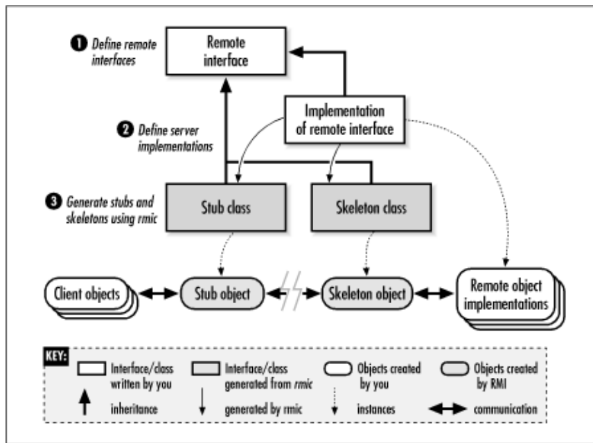
Figure 3–2. Relationships among remote object, stub, and skeleton classes
