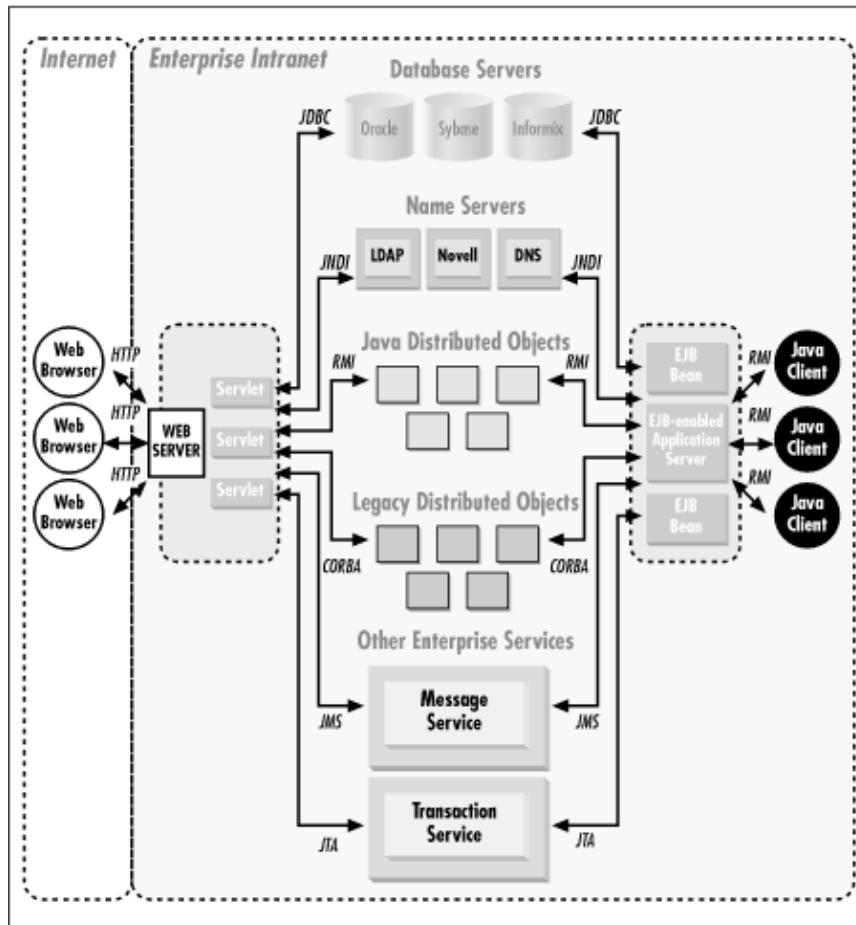
Figure 1-1. The distributed computing architecture of a hypothetical enterprise
