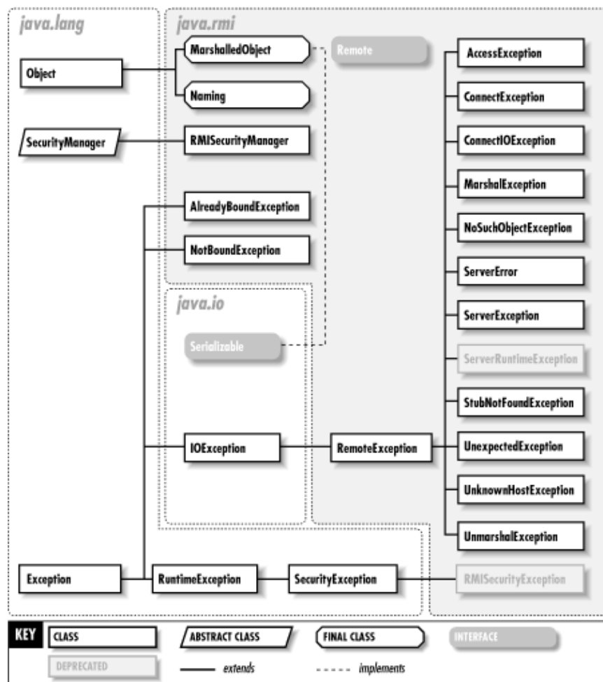
Figure 13–1. The java.rmi package
