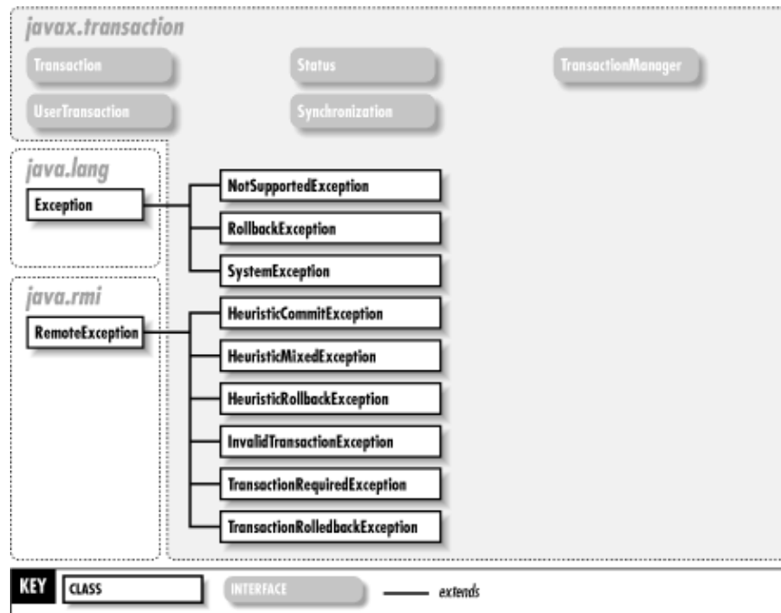
Figure 28–1. The javax.transaction package
