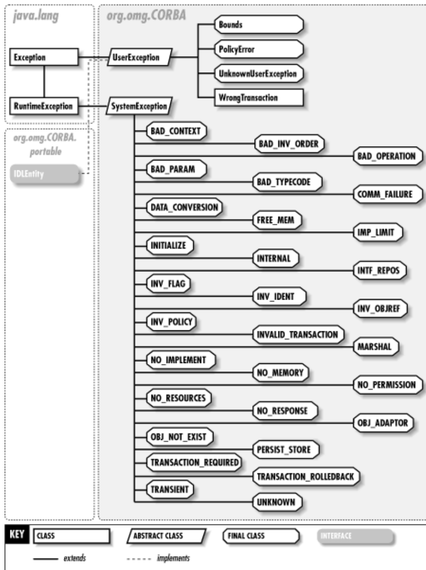
Figure 30–3. The exceptions in the org.omg.CORBA package
