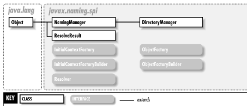
Figure 24–1. The javax.naming.spi package
