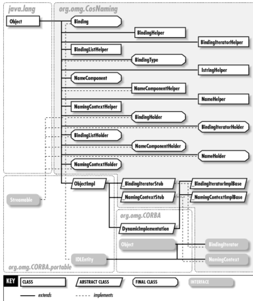
Figure 35–1. The org.omg.CosNaming package
