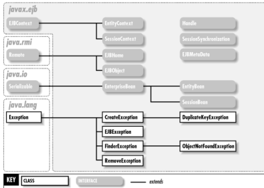
Figure 19-1. The javax.ejb package
