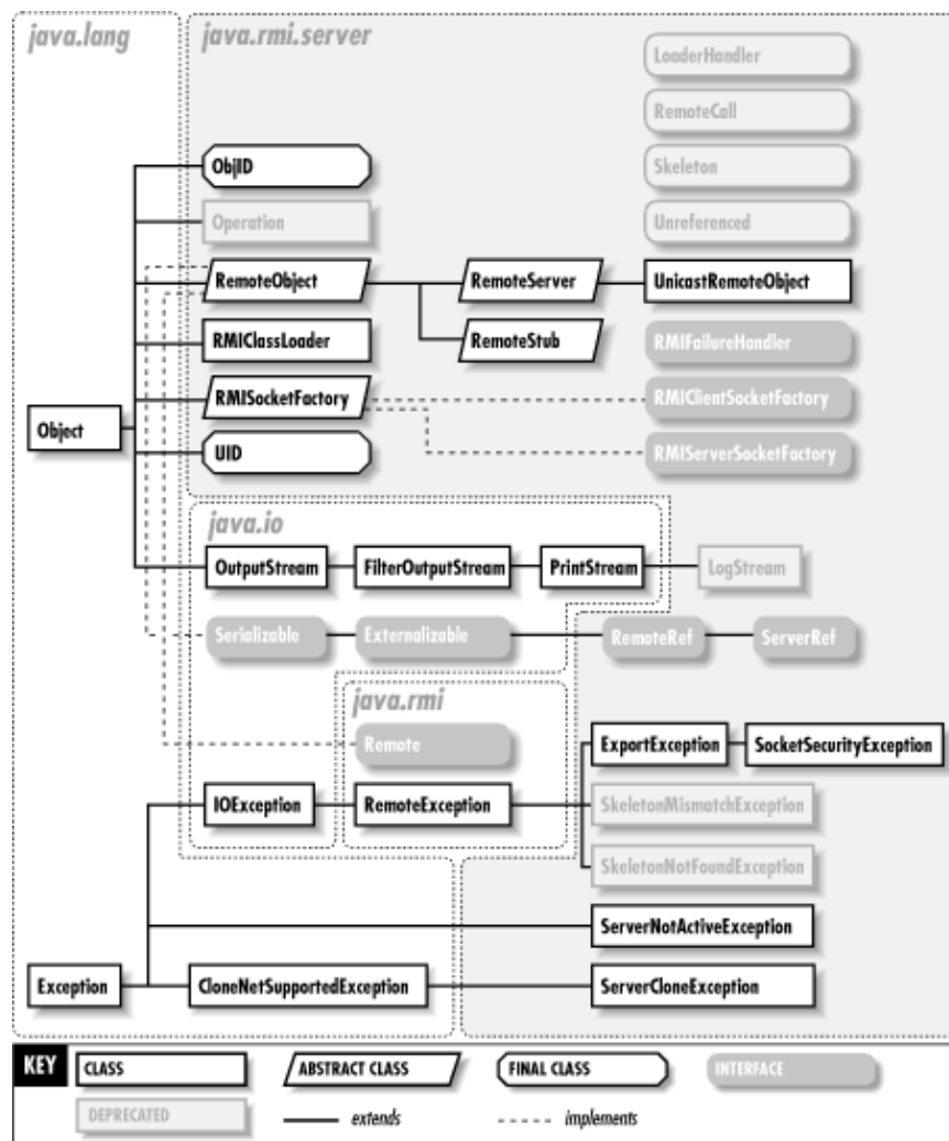
Figure 17–1. The java.rmi.server package
