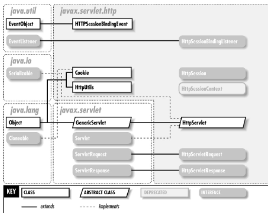
Figure 26–1. The javax.servlet.http package
