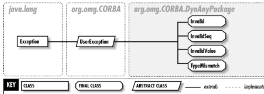
Figure 31–1. The org.omg.CORBA.DynAnyPackage package
