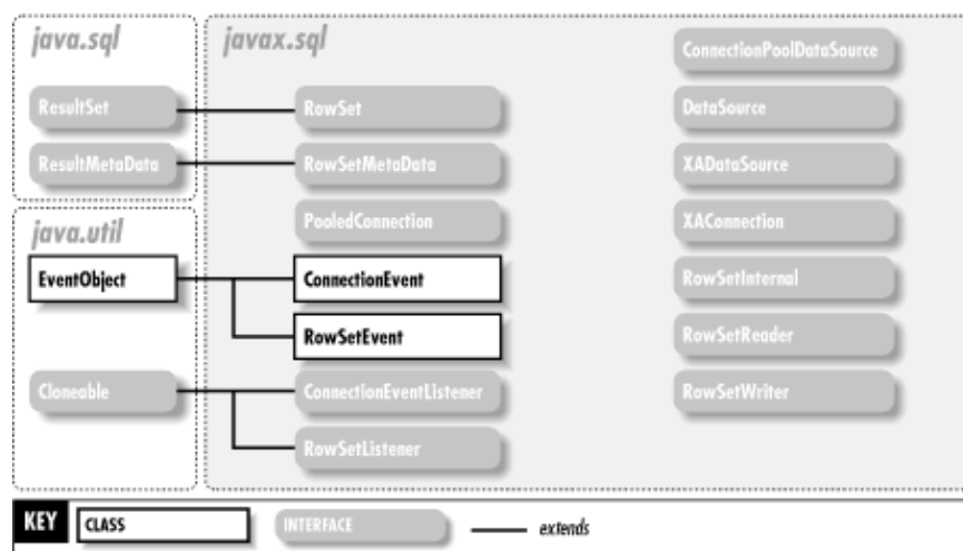
Figure 27-1. The javax.sql package
