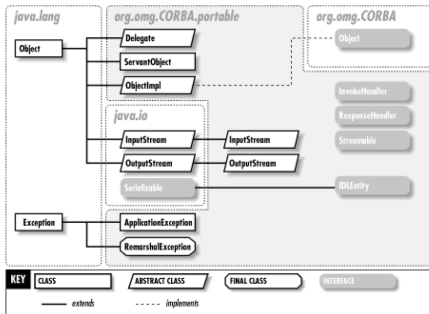
Figure 33–1. The org.omg.CORBA.portable package
