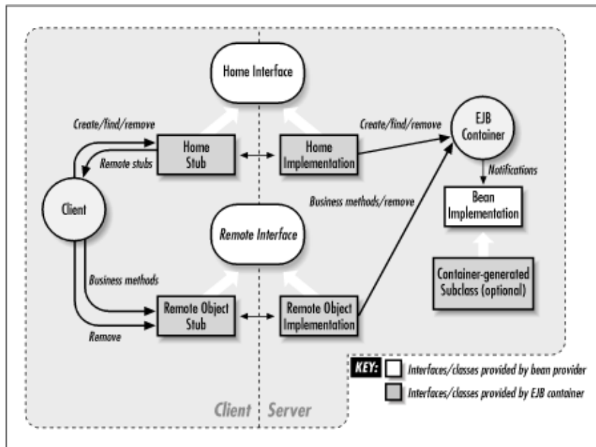
Figure 7-2. Relationship of bean-provider classes and container-generated classes
