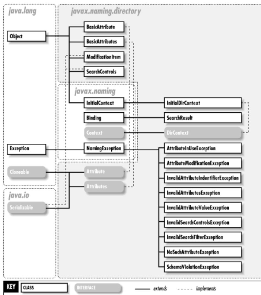
Figure 23–1. The javax.naming.directory package
