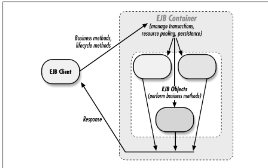
Figure 7-1. The basic roles in an EJB environment
