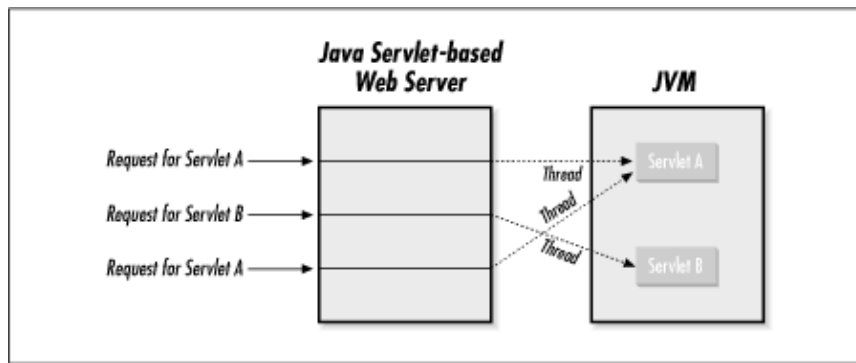
Figure 5–1. The servlet life cycle
