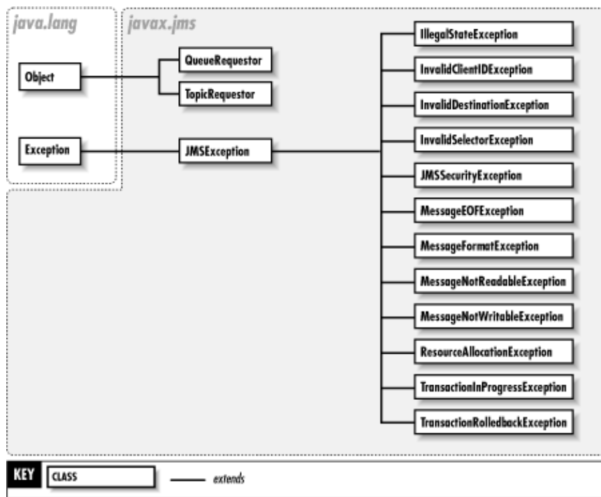
Figure 21–2. The classes and exceptions of the javax.jms package
