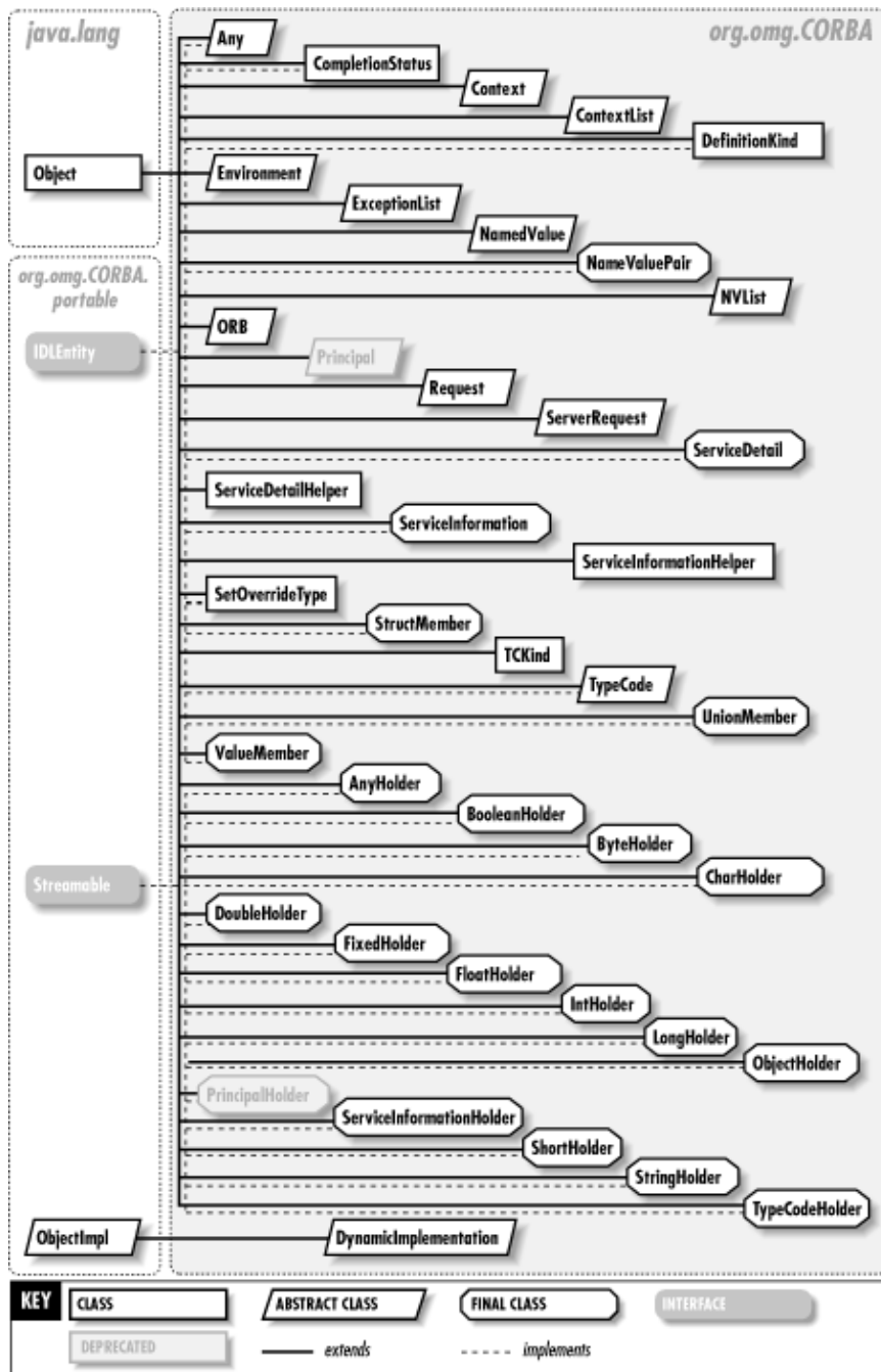
Figure 30–2. The classes in the org.omg.CORBA package
