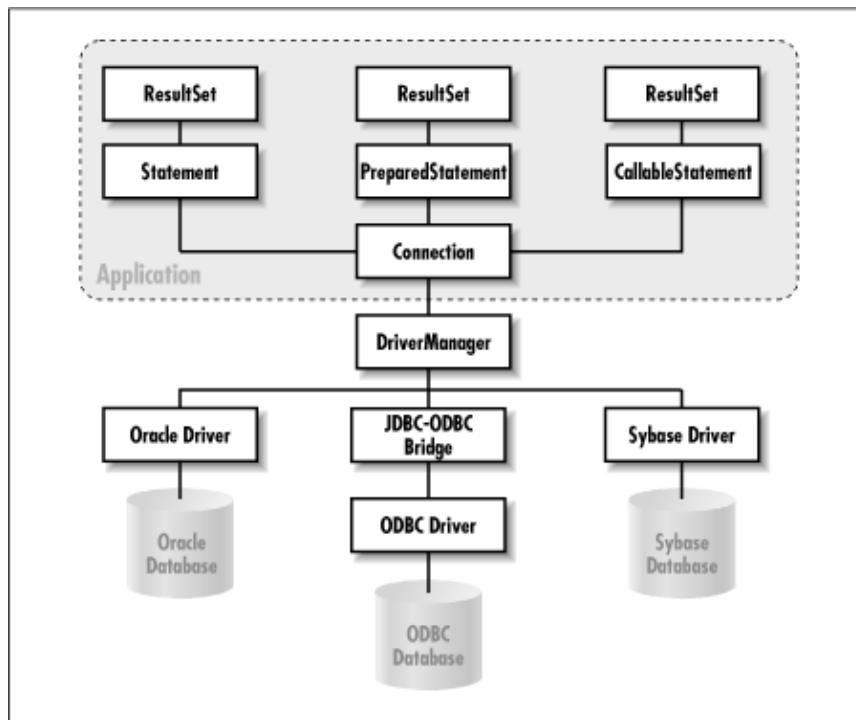
Figure 2–1. JDBC–database interaction
