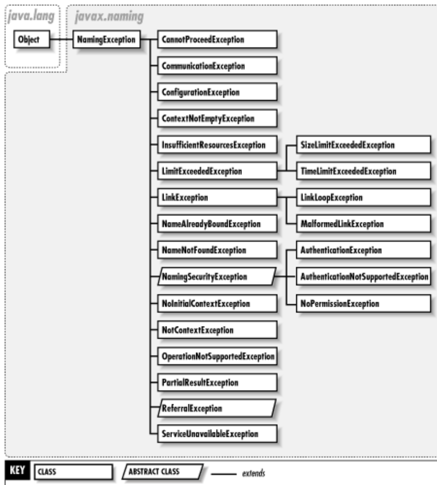
Figure 22–2. The exception hierarchy of the javax.naming package
