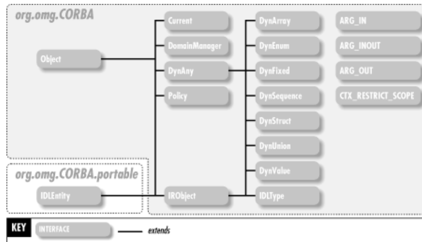
Figure 30-1. The interfaces in the org.omg.CORBA package
