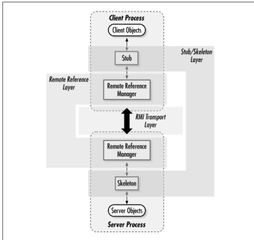
Figure 3–1. The RMI runtime architecture
