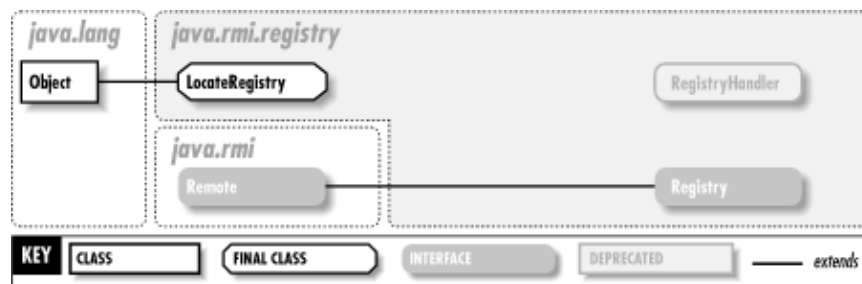
Figure 16–1. The java.rmi.registry package
