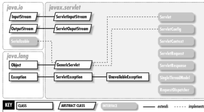
Figure 25–1. The javax.servlet package
