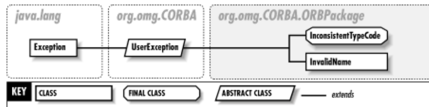
Figure 32–1. The org.omg.CORBA.ORBPackage package
