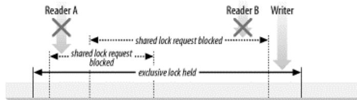
Figure 1-8. Shared-lock requests blocked by exclusive lock
