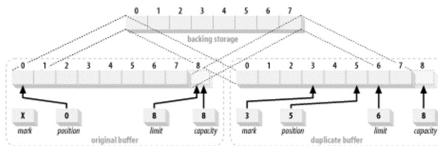
Figure 2-12. Duplicating a buffer
