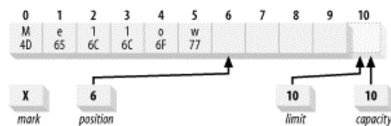
Figure 2-4. Buffer after modification
