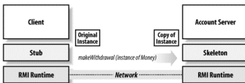
Figure 10-3. Making a remote method call can create deep copies of the arguments and return values
