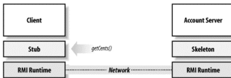
Figure 10-2. Relaying a Money method call from the server
