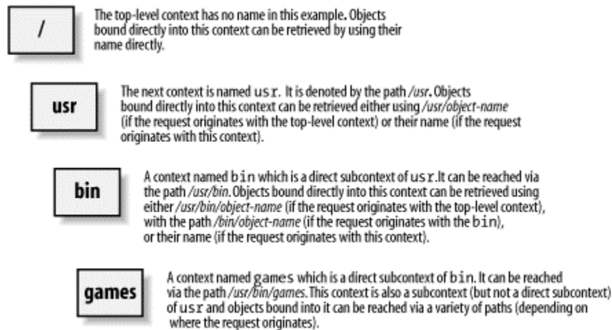
Figure 15-2. Contexts and paths
