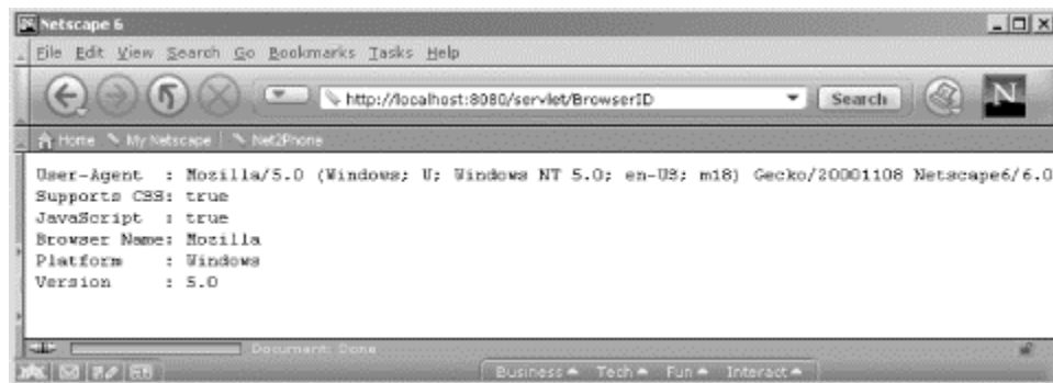
Figure 8-4. Browser detection
