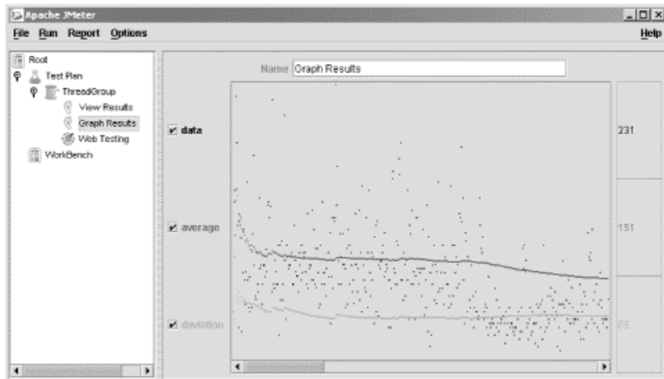
Figure 9-8. JMeter output
