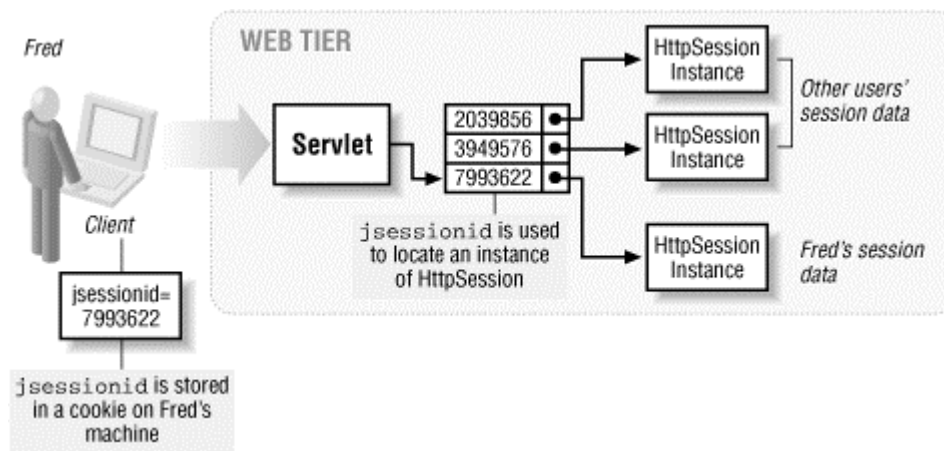
Figure 8-3. Session tracking
