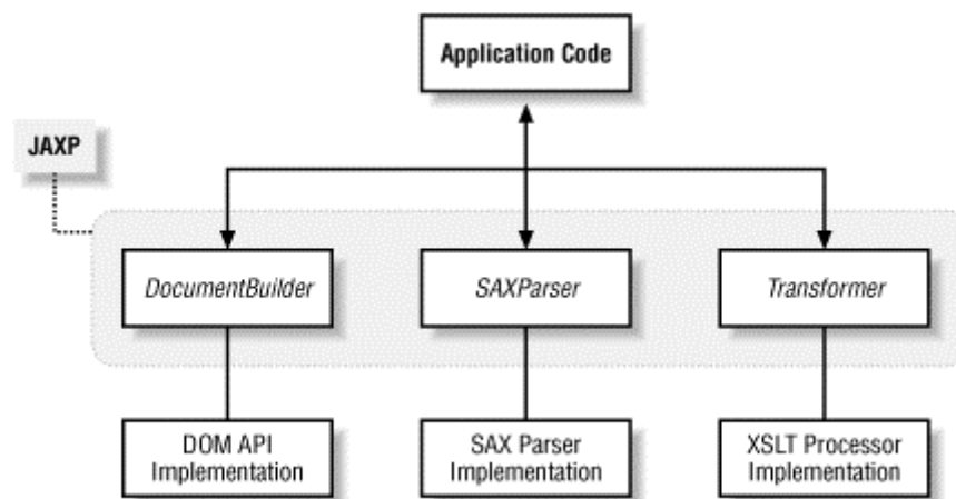
Figure 5-1. JAXP 1.1 architecture
