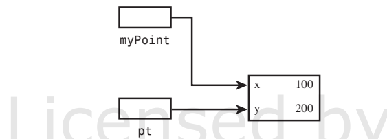
Figure 8.6 Passing the rectangle's origin to the method
