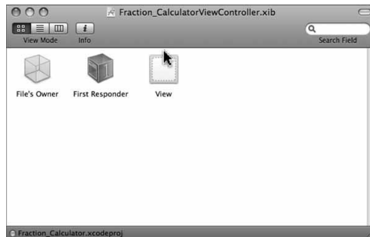
Figure 21.23 Fraction_CalculatorViewController.xib window.
