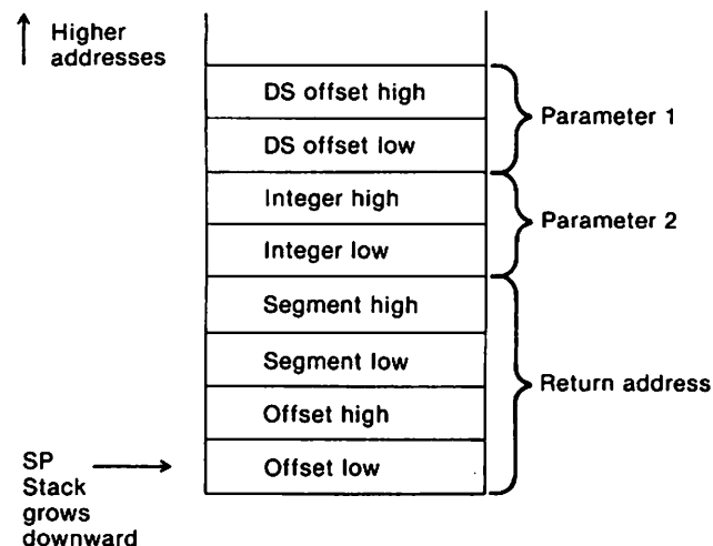
Figure 9.2. Stack Before Transfer to ADD
