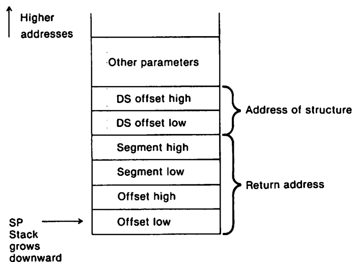
Figure 9.5. Four-Byte Return Value
