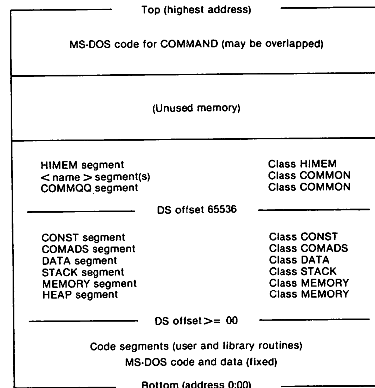
Figure 10.3. Memory Organization
