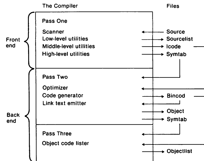
Figure 10.1. The Structure of the Microsoft Pascal Compiler
