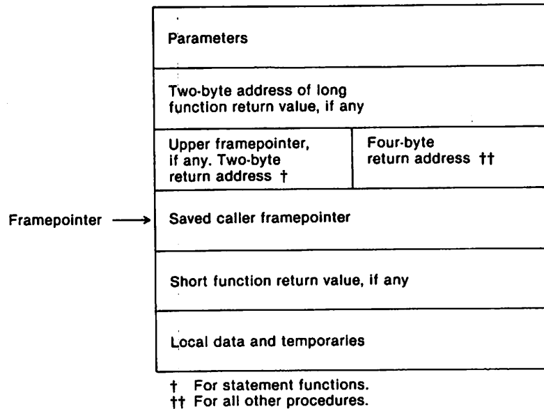
Figure 9.1. Contents of the Frame
