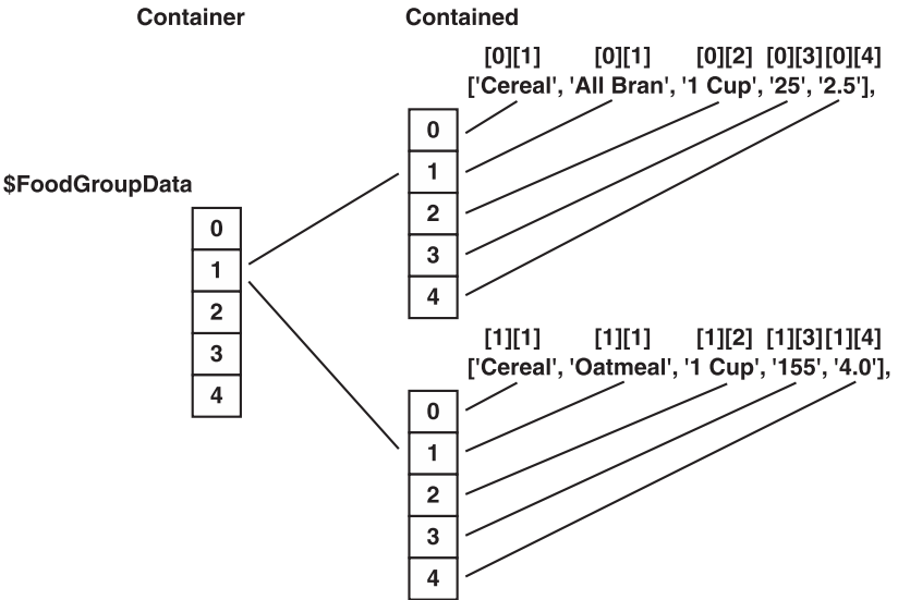
Figure 13.11 An outer container array involves two sets of indexes.
