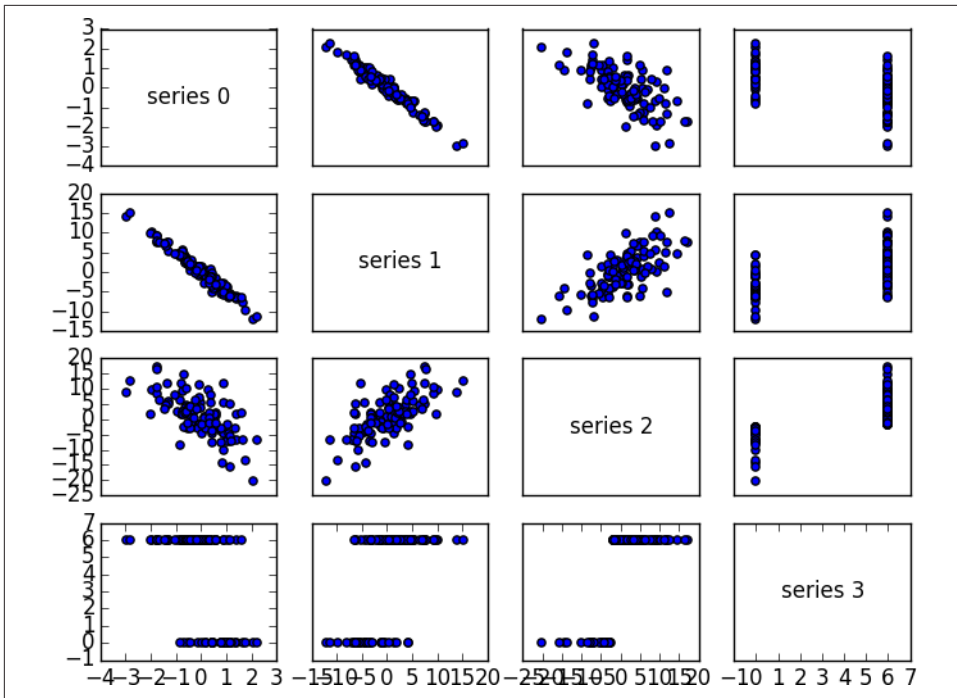
Figure 10-4. Scatterplot matrix
