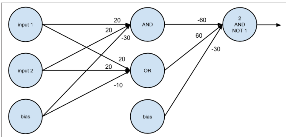
Figure 18-3. A neural network for XOR
