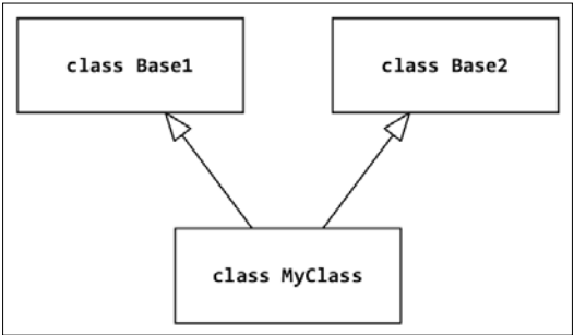
Figure 1 Classical hierarchy
