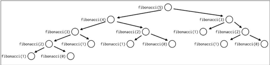
Figure 3 Call tree for fibonacci(5) execution
