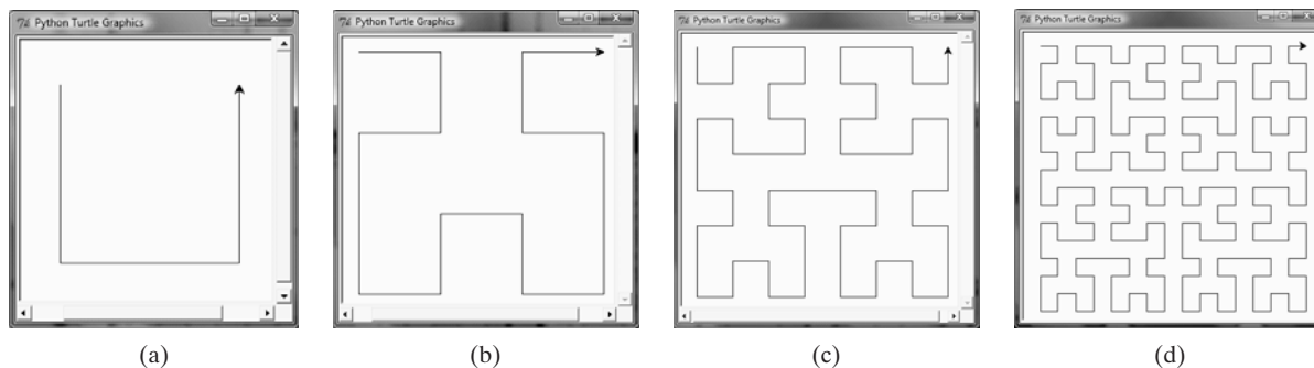
FIGURE 15.20 A Hilbert curve is drawn using Turtle with order 0 in (a), 1 in (b), 2 in (c), and 3 in (d).
