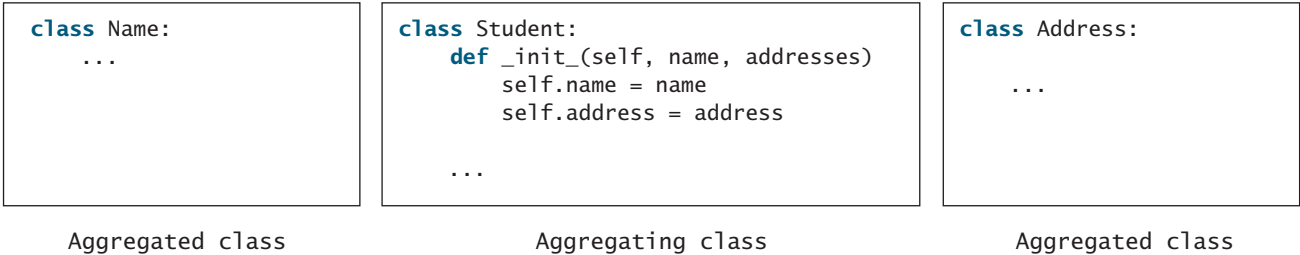
FIGURE 12.8 The composition relations are implemented using data fields in classes.
