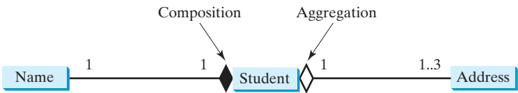
FIGURE 12.7 Each student has a name and an address.
