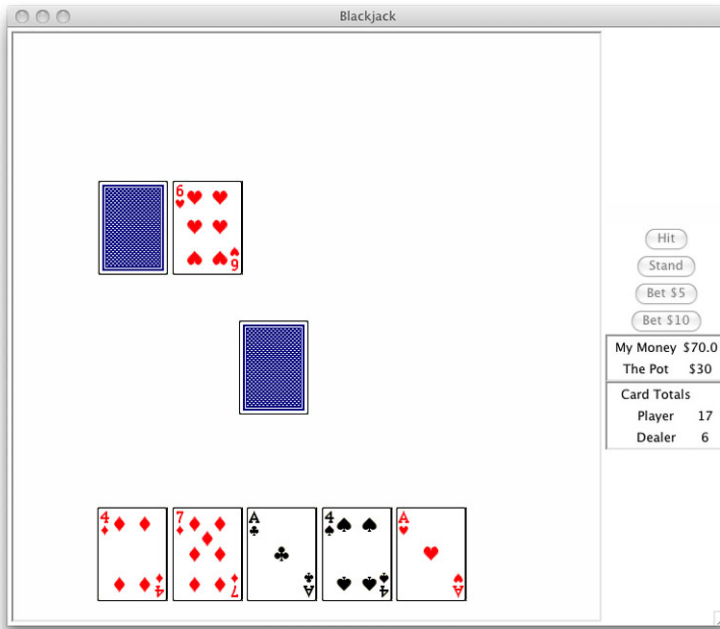
Fig. 7.6 A Blackjack Hand
