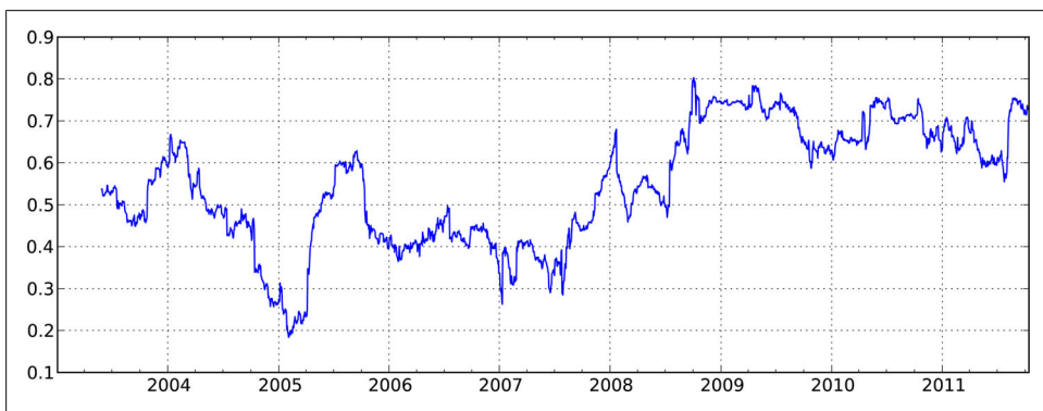
Figure 10-12. Six-month AAPL return correlation to S&P 500
