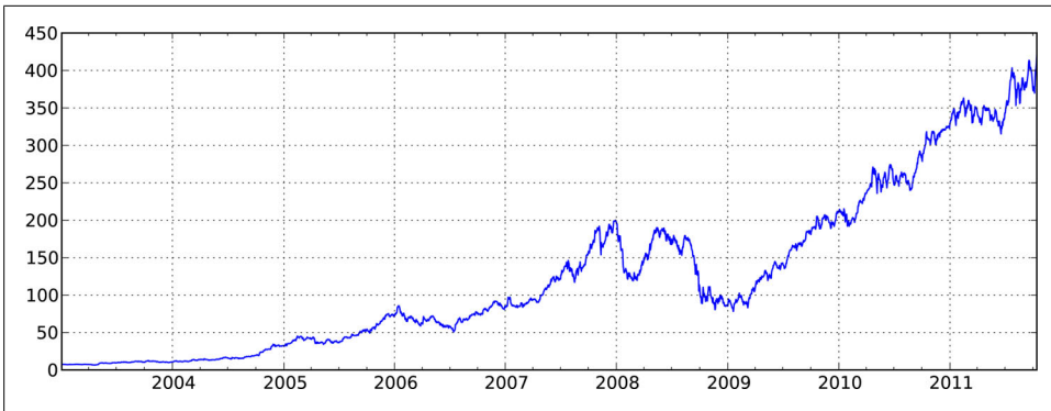
Figure 10-4. AAPL Daily Price
