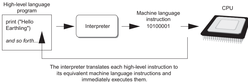
Figure 1-20 Executing a high-level program with an interpreter
