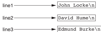
Figure 7-12 The strings referenced by the line1 , line2 , and line3 variables
