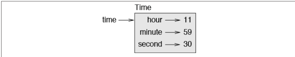
Figure 16-1. Object diagram.
