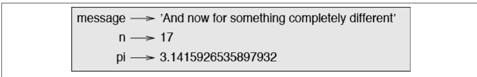
Figure 2-1. State diagram.
