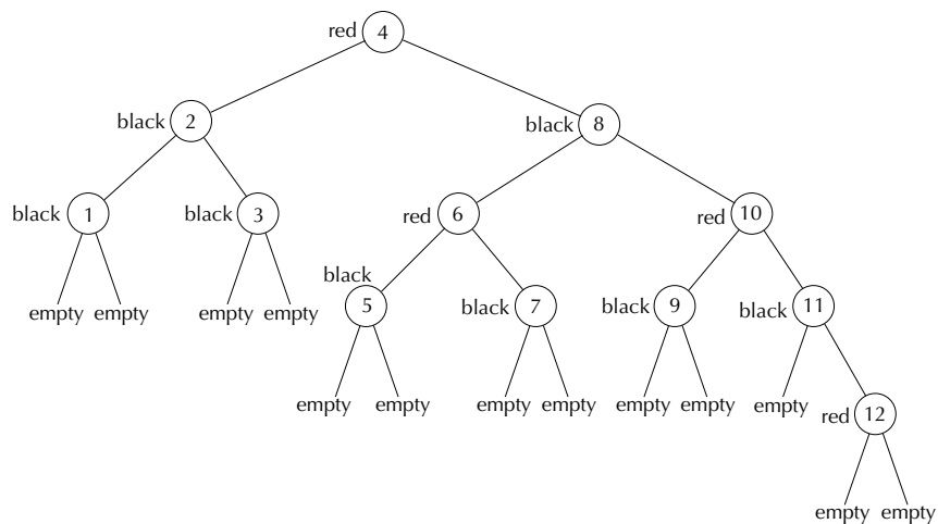
Figure 13.11 A red-black tree containing numbers
