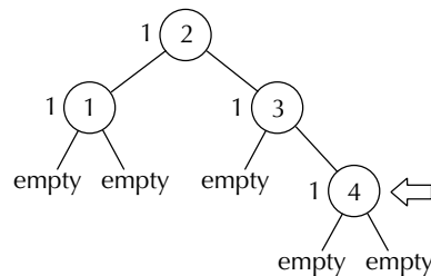
Figure 13.18 Inserting 1, 2, 3, and 4 into an empty red-black tree
