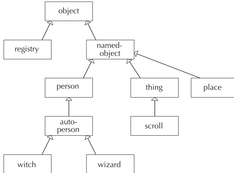
Figure 14.1 The class hierarchy for the Land of Gack
