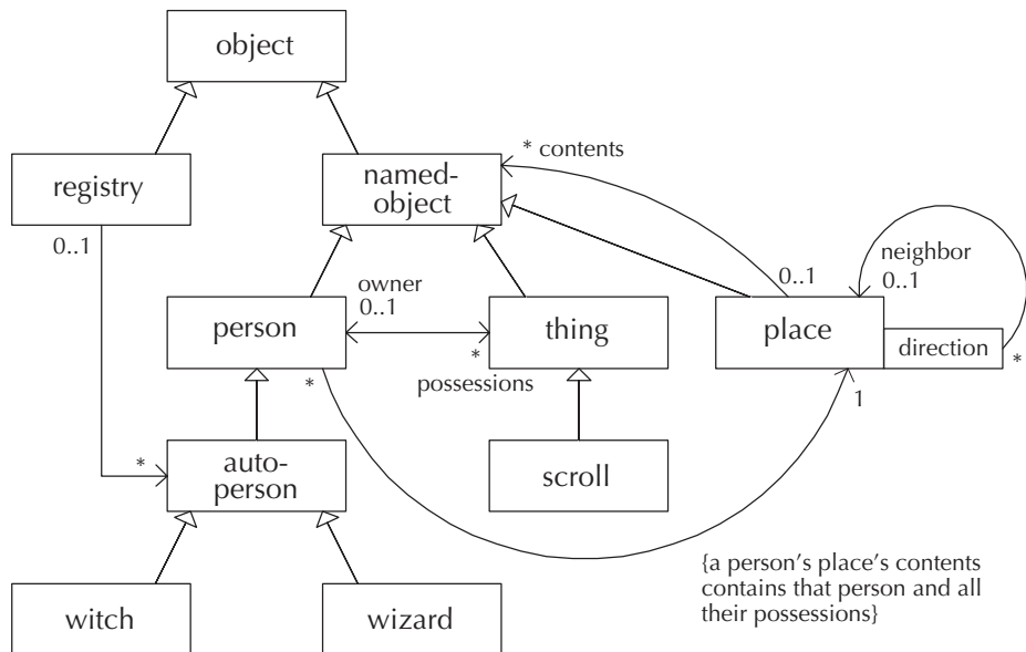
Figure 14.2 The Land of Gack class diagram, including associations
