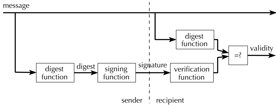
Figure 4.2 The full digital signature system, including the digest function
