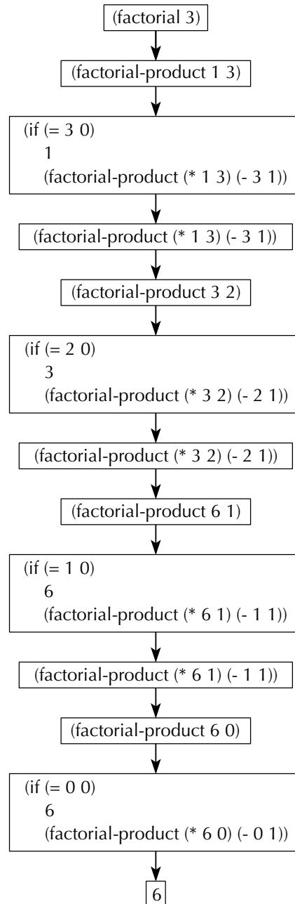
Figure 3.1 The iterative process of evaluating (factorial 3) .
