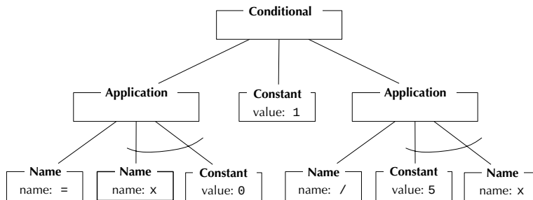
Figure 10.1 Conditional AST parsed from (if (= x 0) 1 (/ 5 x))
