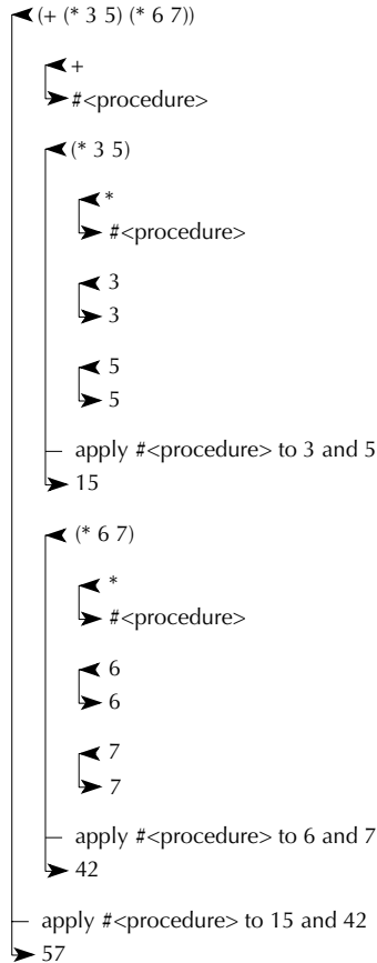
Figure 10.11 Explanatory output with applications shown
