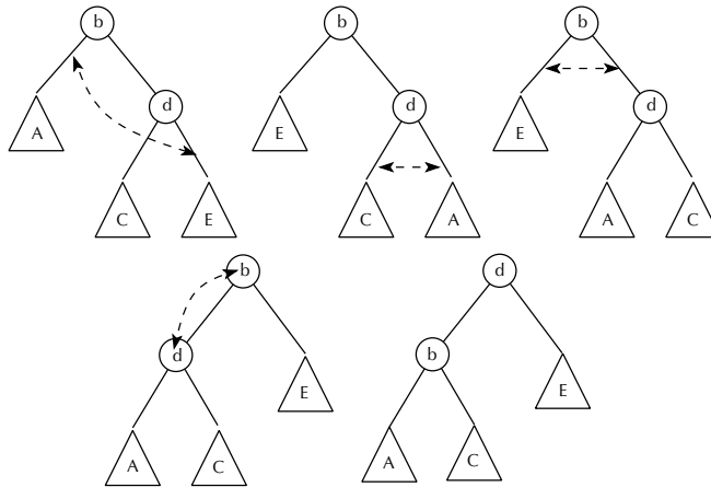
Figure 13.26 Left rotation through a sequence of exchanges
