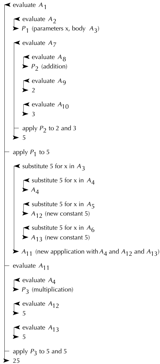
Figure 10.5 The process of evaluating the AST A_1
