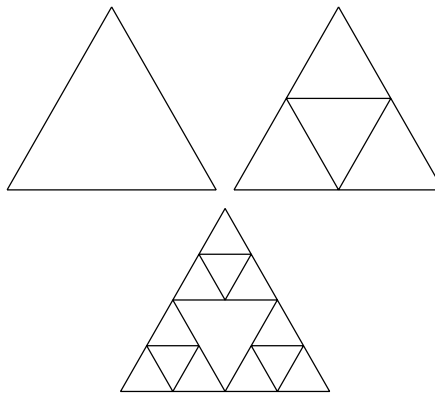
Figure 4.8 Sierpinski's gaskets of levels 0, 1, and 2.
