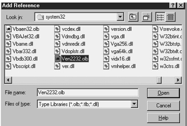
FIGURE 10.2 You can browse for the file containing a component's Object Library if the component isn't listed in the Available References list of the References dialog box.
