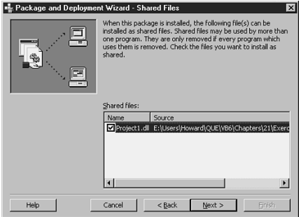
FIGURE 21.12▲ Package and Deployment Wizard's Shared Files dialog box.
