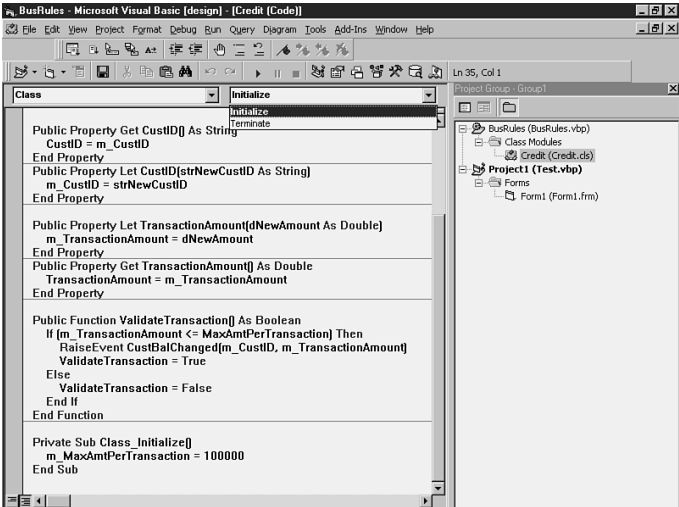
FIGURE 12.4 Navigating to a class module's Initialize and Terminate event procedures.
