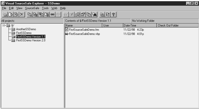
FIGURE 2.26► A project that shows a branched file (no longer pinned).
