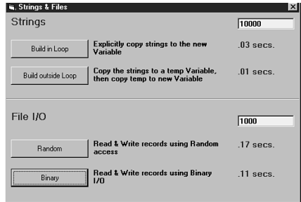
FIGURE 20.11▲ Results of the string manipulation and file I/O test when compiling native code with no optimizations.
