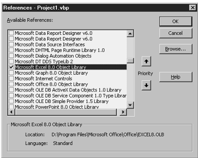
FIGURE 10.1 Use the References dialog box to set a reference in your project to a COM component.
