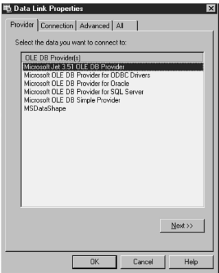
FIGURE 8.4▲ Choosing the provider for a Connection object in the Data Environment Designer.
