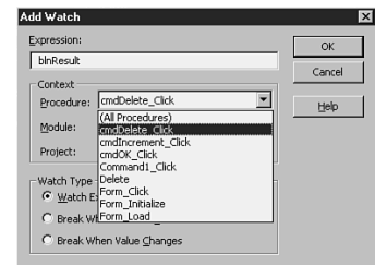
FIGURE 18.24 A procedure-level watch.
