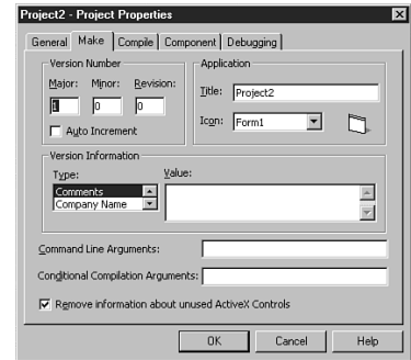
FIGURE 4.18▲ The Make tab of the Project Properties dialog showing the option that controls references to unused ActiveX controls.
