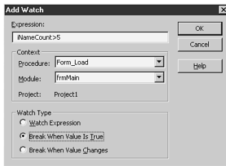
FIGURE 18.11 Select Break When Value Is True to enter Break mode automatically when a value is True.
