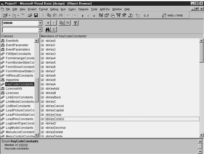
FIGURE 5.1 Finding the names of VB KeyCode constants in the Object Browser.
