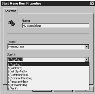
FIGURE 21.10▲ Specifying the properties for your application's Start menu icon.
