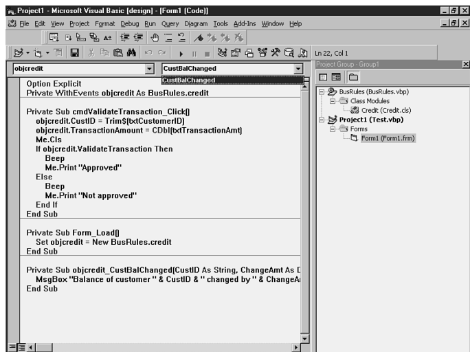
FIGURE 12.5 Navigating to the event procedure for a custom object's event.
