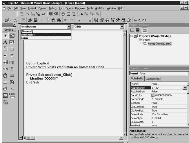
FIGURE 4.16 Once you've declared your control using WithEvents , you can see the control and its events in the drop-down lists of the Code window.
