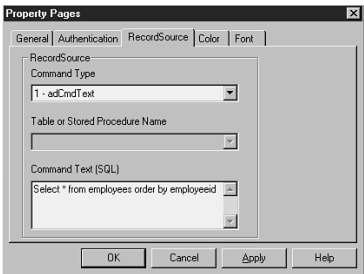
FIGURE 8.19▲ A valid Select statement as command text for the RecordSource property.
