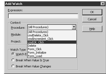
FIGURE 18.5▲ You can also limit the scope of a Watch expression to a particular procedure.
