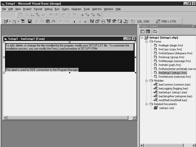
FIGURE 21.17 You can customize an application’s setup routine by opening and modifying SETUP1.VBP. The designer for frmSetup1 is shown here.
