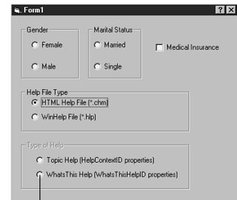
WhatsThisButton
