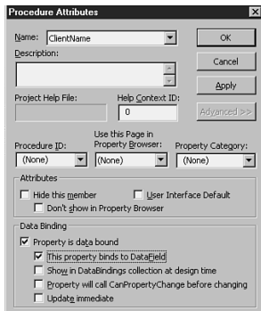
FIGURE 13.7 Specifying a property to bind to the DataField .
