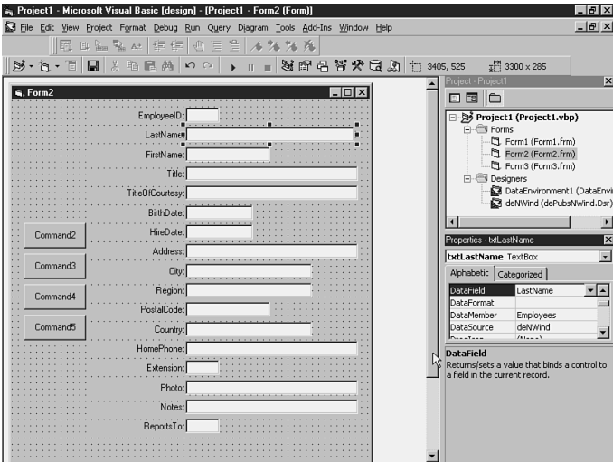
FIGURE 8.11▲ Dropping a Command object from a Data Environment Designer onto a form to create a control bound to an entire Recordset. This figure shows both the dialog box at the instant you drop the object and the result of the drop.
