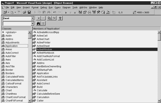
FIGURE 10.3▶ The Object Browser can give you detailed information about a COM component's objects and their methods and properties.
