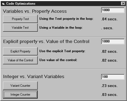
FIGURE 20.14▲ Results of the code optimizations test when compiling to native code optimized for size.
