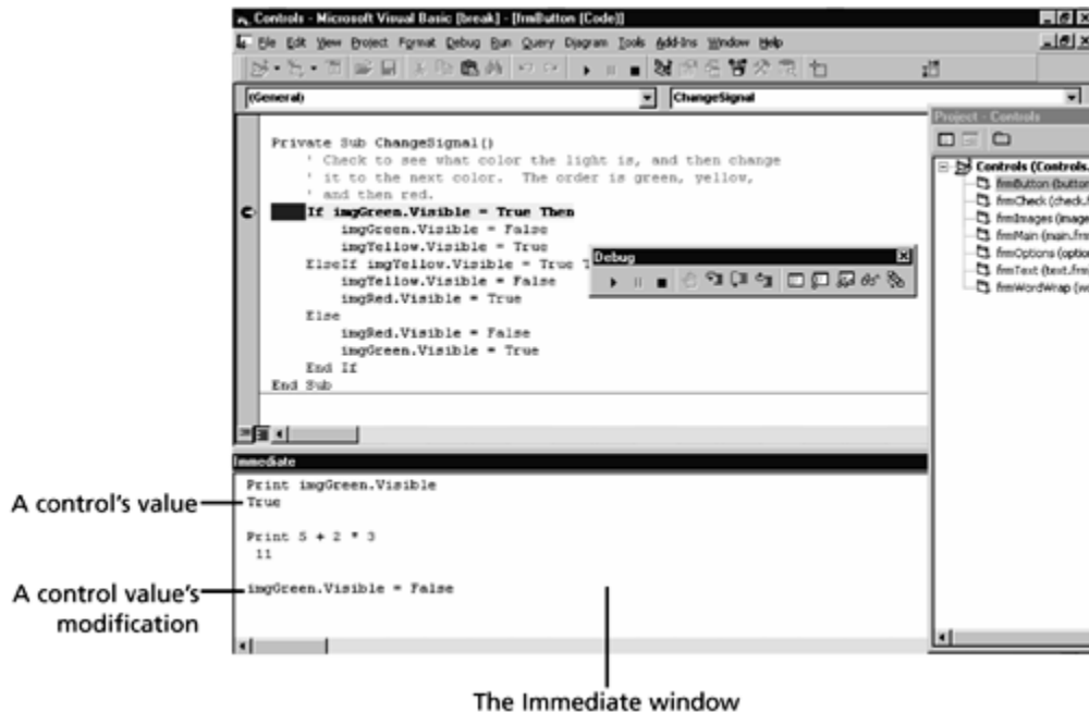
Figure 21.6. Using the Immediate window to print values and change results.
