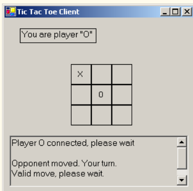
Fig. 22.7 Client side of client/server Tic-Tac-Toe program (part 6 of 7).
