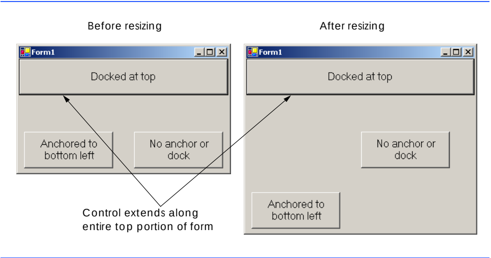
Fig. 12.13 Docking demonstration.
