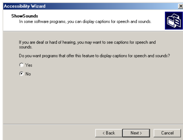
Fig. 24.30 ShowSounds dialog.
