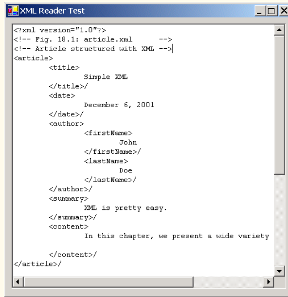
Fig. 18.7 XmlNodeReader iterates through an XML document (part 3 of 3).
