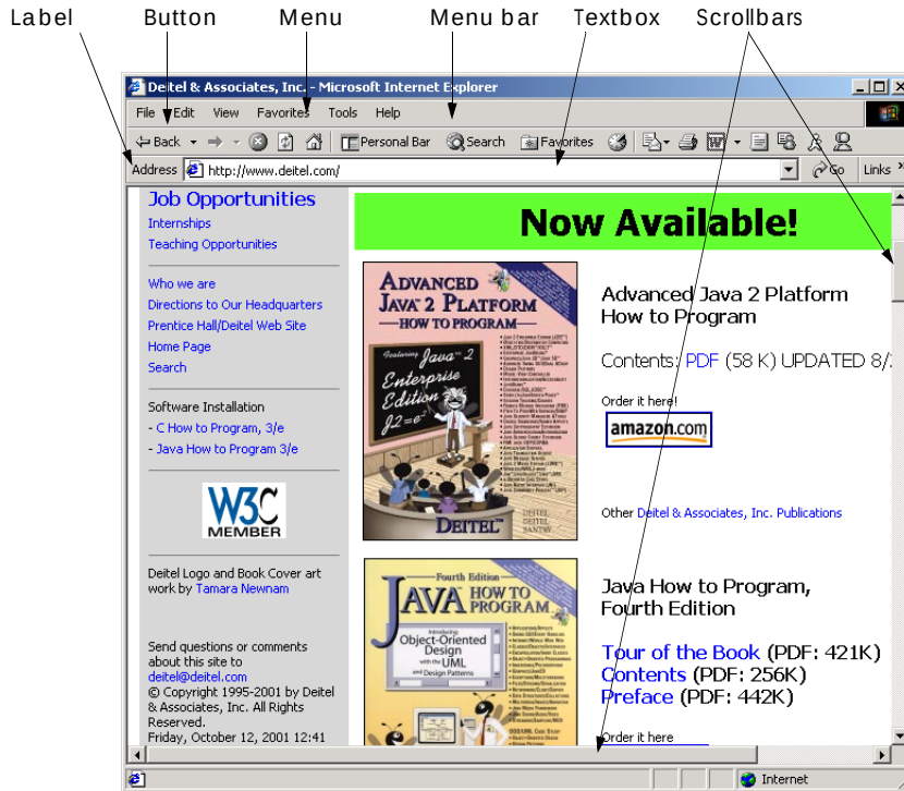
Fig. 12.1 GUI components in a sample Internet Explorer window.
