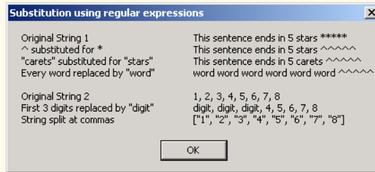
Fig. 15.23 Regex methods Replace and Split (part 3 of 3).
