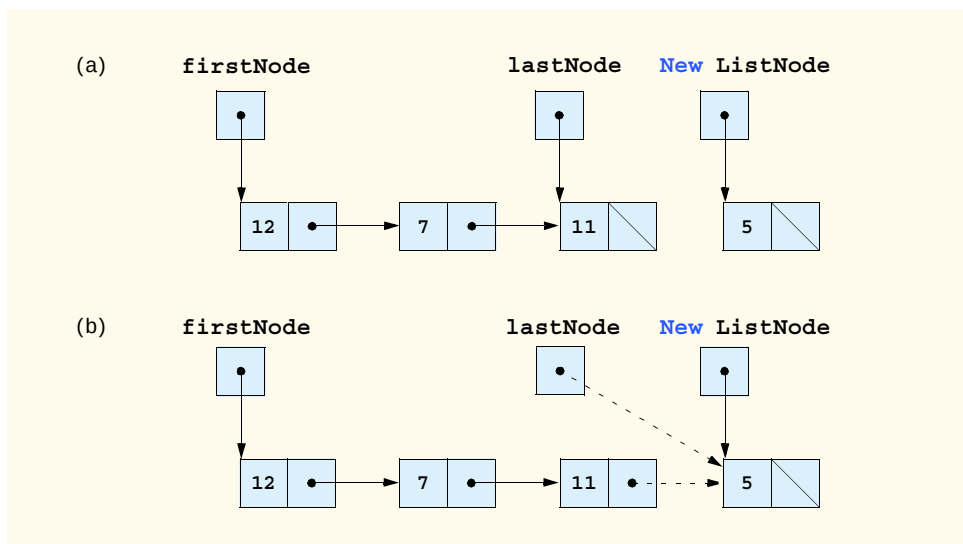
Fig. 23.9 InsertAtBack graphical representation.
