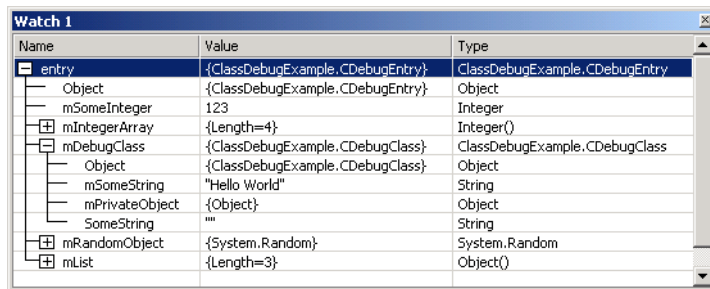
Fig. D.23 Expanded class in Watch window.
