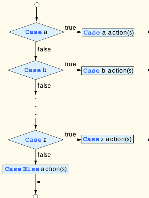
Fig. 5.11 Select Case multiple-selection structure flowchart.
