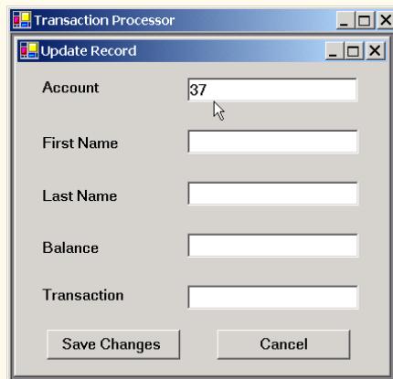
Fig. 17.22 FrmUpdateDialog class enables users to update records in transaction-processor case study (part 5 of 6).
