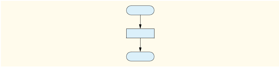
Fig. 5.26 Simplest flowchart.
