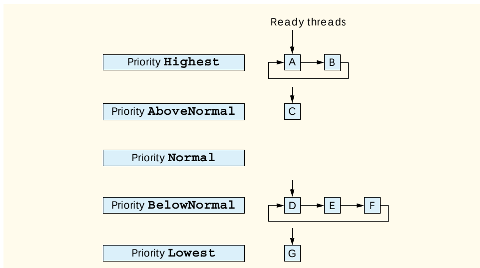
Fig. 14.2 Thread-priority scheduling.
