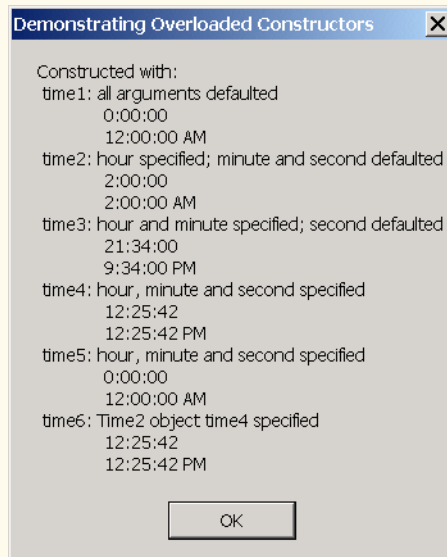
Fig. 8.5 Overloaded-constructor demonstration (part 2 of 2).
