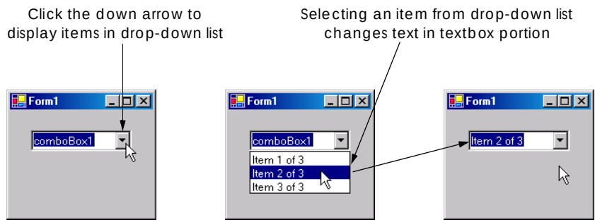
Fig. 13.15 ComboBox demonstration.
