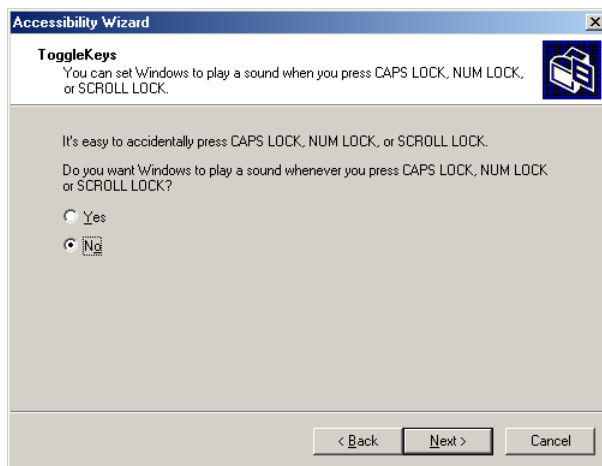
Fig. 24.33 ToggleKeys window.
