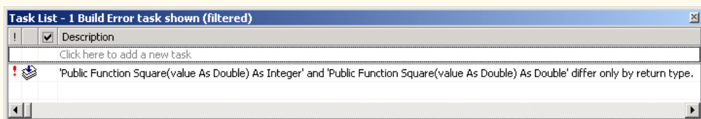
Fig. 6.23 Syntax error generated from overloaded procedures with identical parameter lists and different return types.
