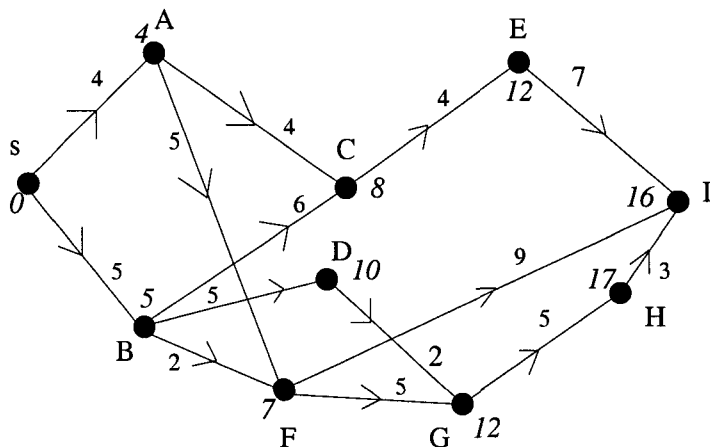
Fig. 17.3 The Output of the Dijkstra algorithm.
