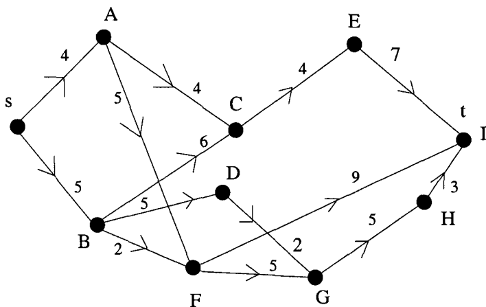
Fig. 17.2 We will use the Dijkstra algorithm on this graph.
