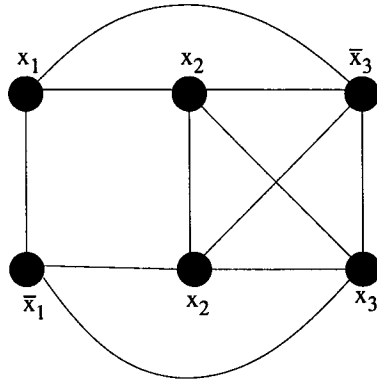
Fig. 18.4 The graph G_B of B = (x_1 \vee x_2 \vee \bar{x}_3) \wedge \bar{x}_1 \vee x_2 \vee x_3 .
