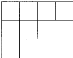
Fig. 5.1 The Ferrers shape of the partition p = (4, 2, 1) .
