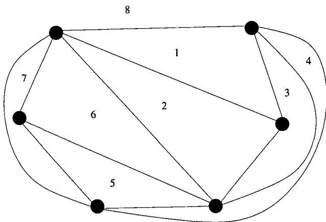
Fig. 12.2 This graph has eight faces.
