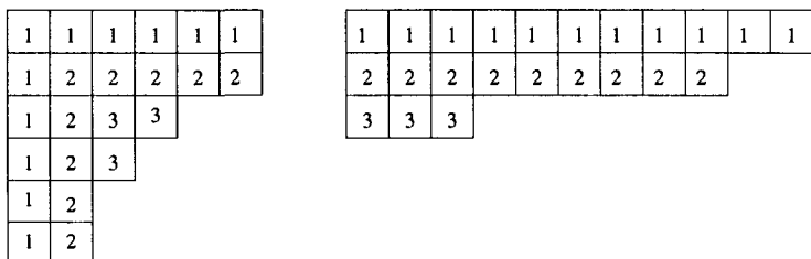
Fig. 5.3 A self-conjugate partition and its image.
