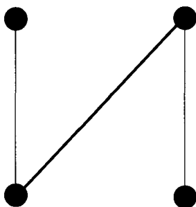
Fig. 11.5 A maximal, but not maximum, matching.
