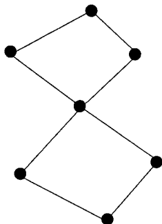
Fig. 9.13 A graph with no Hamiltonian cycle.
