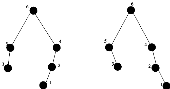
Fig. 14.7 Trees T(p) and T(f(p)) .
