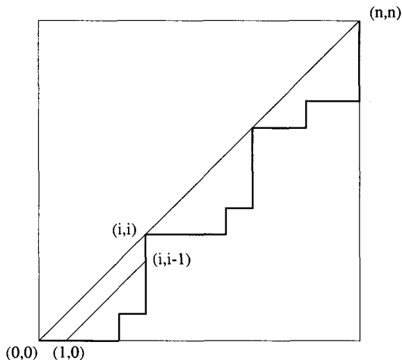
Fig. 14.2 Decomposing our lattice paths.
