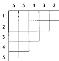
Fig. 5.5 Numbering the rows and columns of the staircase shape.
