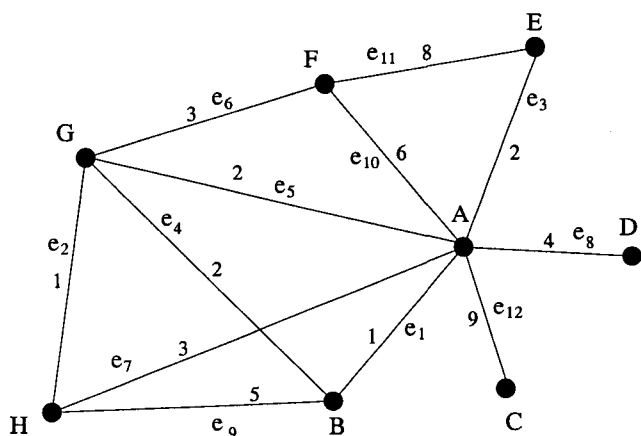
Fig. 17.1 The graph G with its cost function and sorted edges.
