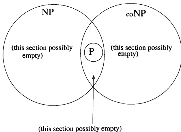
Fig. 18.1 The known inclusions between the three complexity classes defined so far.
