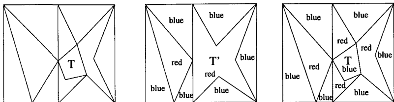
Fig. 12.6 The induction step.
