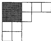
Fig. 5.4 The Durkee square of the partition (5, 3, 2, 2) .
