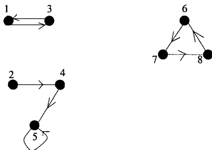
Fig. 10.3 The action of f .
