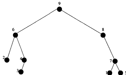
Fig. 14.5 Read in postorder, this tree yields 234615789.
