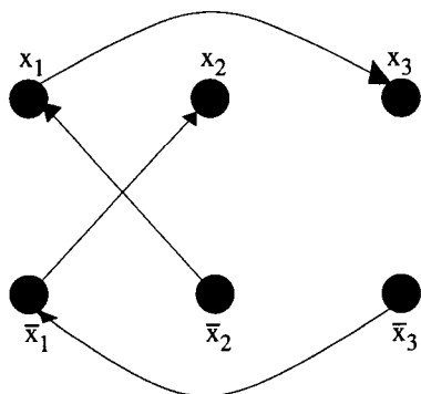
Fig. 18.3 The graph G_B defined by B = (x_1 \vee x_2) \wedge (\bar{x}_1 \vee x_3) .
