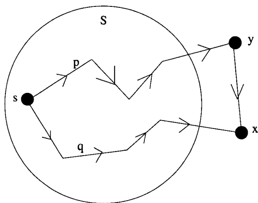
Fig. 17.4 The path p is longer than the path q .
