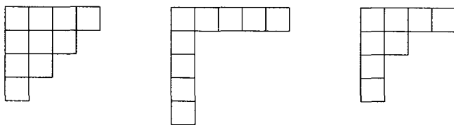
Fig. 5.2 Self-conjugate partitions.
