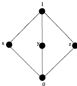
Fig. 16.10 A lattice that is not distributive.
