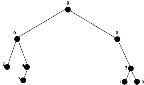
Fig. 14.4 The decreasing binary tree of p = 263498175 .
