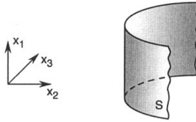
Figure 19.2 A two-dimensional surface in \mathbb{R}^3
