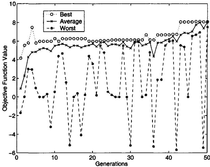
Figure 14.5 The best, average, and worst objective function values in the population for every iteration (generation) of the genetic algorithm in Example 14.3
