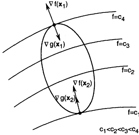
Figure 20.3 Points satisfying the KKT condition ( x_1 is a maximizer and x_2 is a minimizer)
