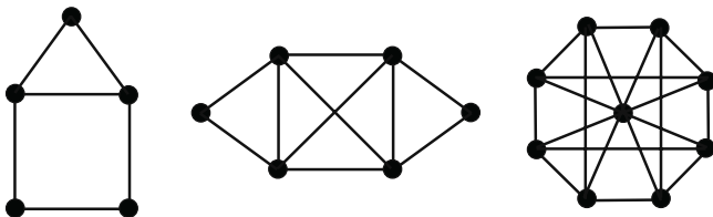
FIGURE 1.54. Are any of these Eulerian?
