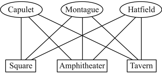
FIGURE 1.72. Original routes.
