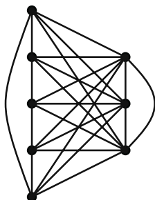
FIGURE 1.92. Is \chi(G) = \omega(G) ?
