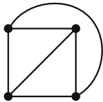
FIGURE 1.74. A planar representation of K_4 .
