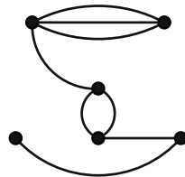
FIGURE 1.4. A multigraph.
