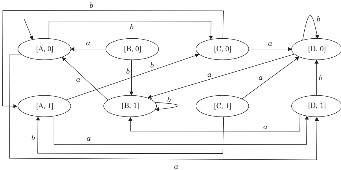
Fig. 9.44 Moore machine.
