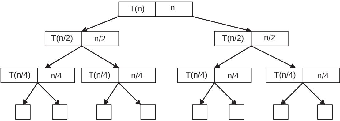
Fig. 3.3 Recursion tree.
