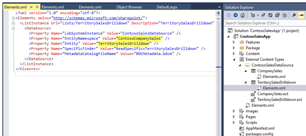
Figure 3-17: Update the Elements.xml file for consistency.
