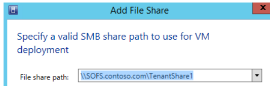
FIGURE 5-19 Selecting TenantShare1
