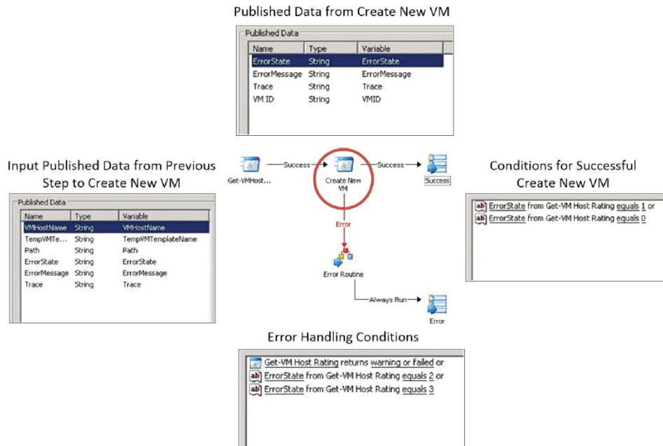
FIGURE 4-10 An example of the Orchestrator activity design pattern.
