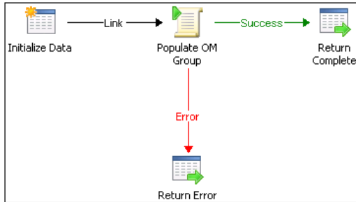
FIGURE 5-16 Component runbook structure.
