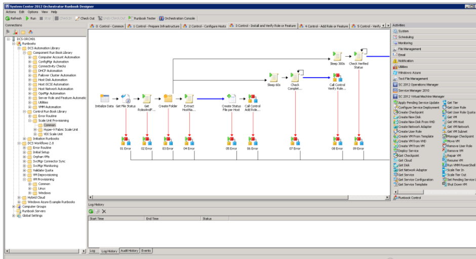
FIGURE 2-1 The Orchestrator Runbook Designer.
