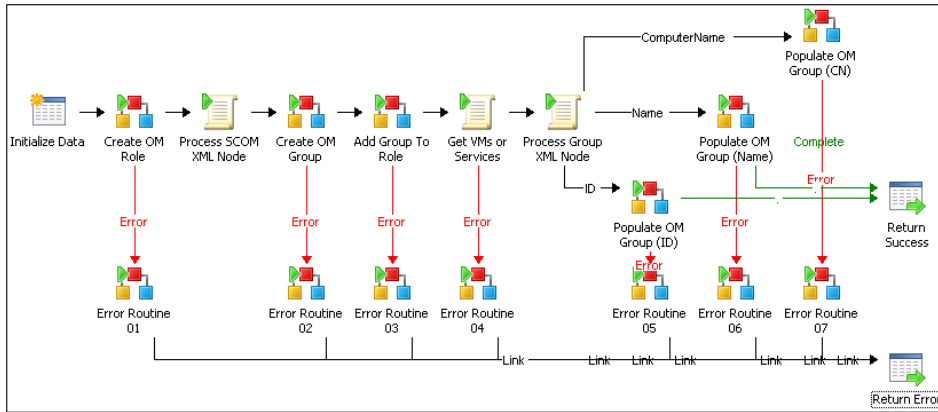
FIGURE 5-17 Control runbook design pattern example.
