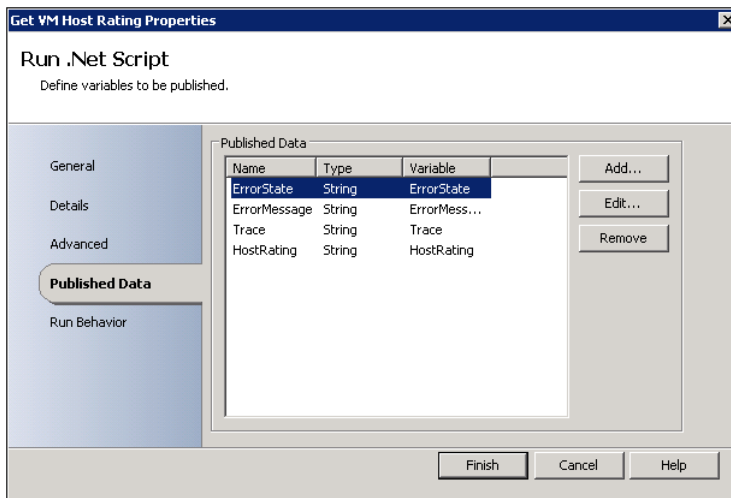
FIGURE 6-4 You can see the defined variable in the Publish Data tab.
