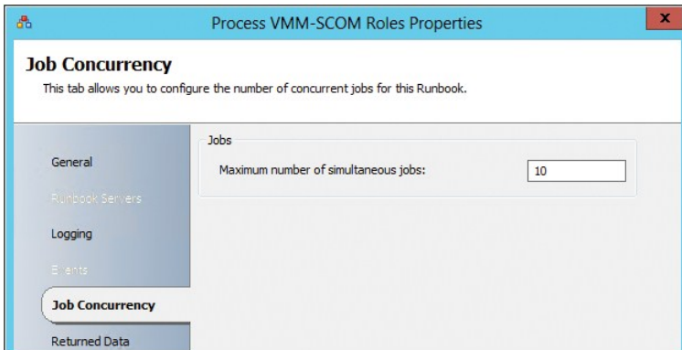
FIGURE 5-13 Setting a runbook's number of simultaneous jobs (job concurrency).
