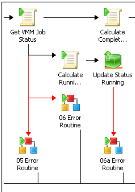
FIGURE 4-2 One activity may have multiple output paths.
