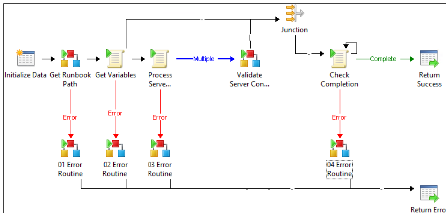
FIGURE 5-30 A local state pattern example.
