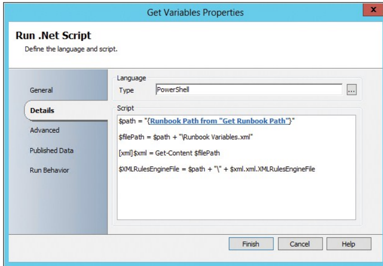
FIGURE 5-26 The Get Variables .Net Script Activity script pane.
