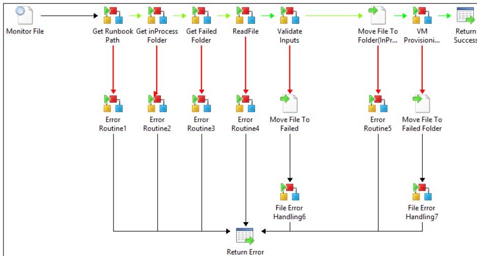
FIGURE 6-10 A diagram of the Monitor VM Provisioning runbook.
