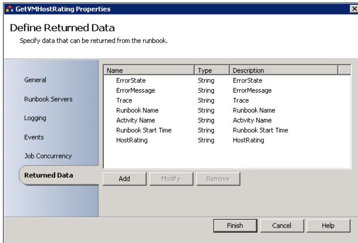
FIGURE 6-5 You can specify the data in the Returned Data tab.
