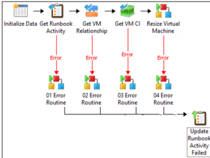
FIGURE 5-23 An example of an initiation runbook to handle a Service Manager service request.
