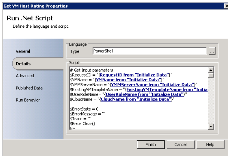
FIGURE 6-3 An example of mapping published data to script.
