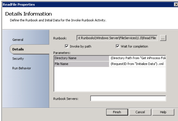
FIGURE 6-13 The Details tab with the Invoke Runbook setting for ReadFile.
