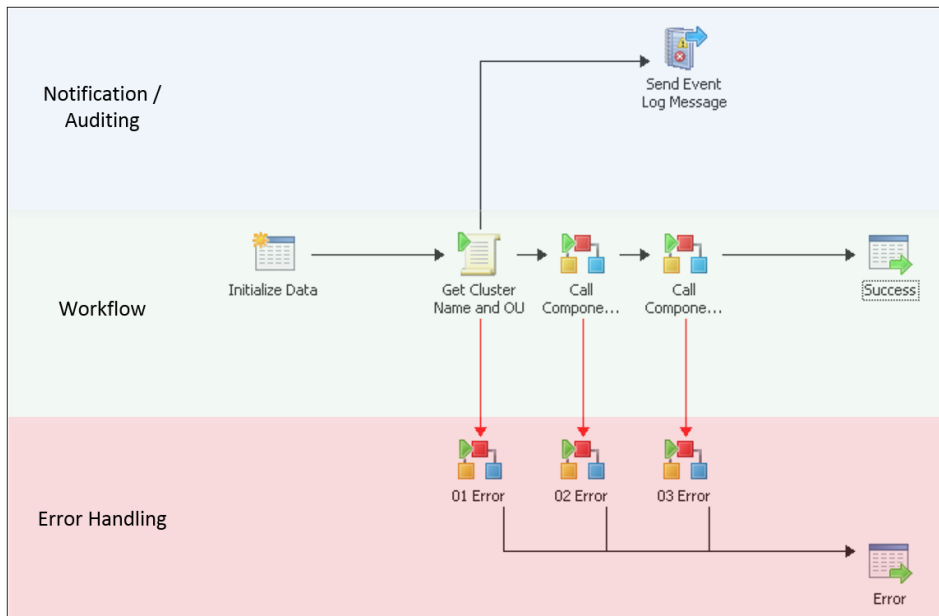
FIGURE 4-6 A runbook that uses the “three rail” design paradigm.
