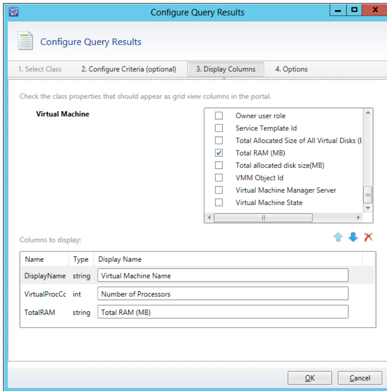
FIGURE 7-22 The Display Columns tab of the Configure Query Results Wizard.
