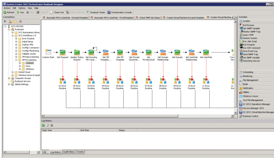
FIGURE 4-1 The System Center Orchestrator Runbook Designer.
