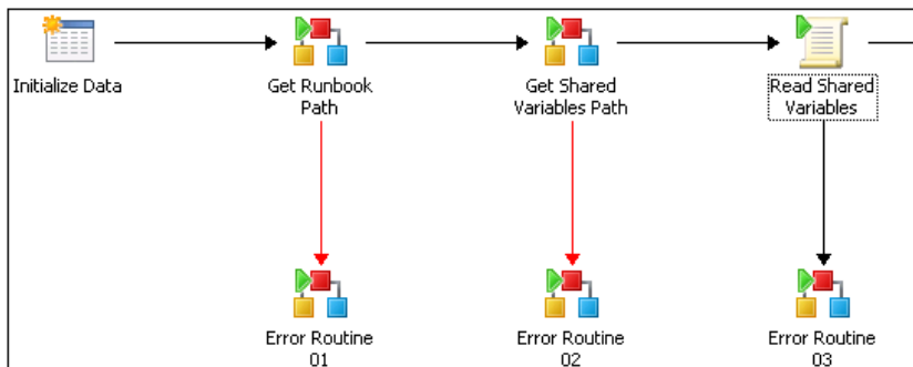
FIGURE 5-28 Adding the Get Relative Folder runbook for shared variable access.
