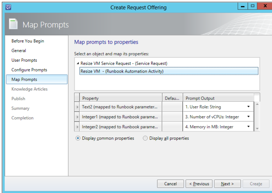
FIGURE 7-24 The Map Prompts page of the Create Request Offering Wizard.
