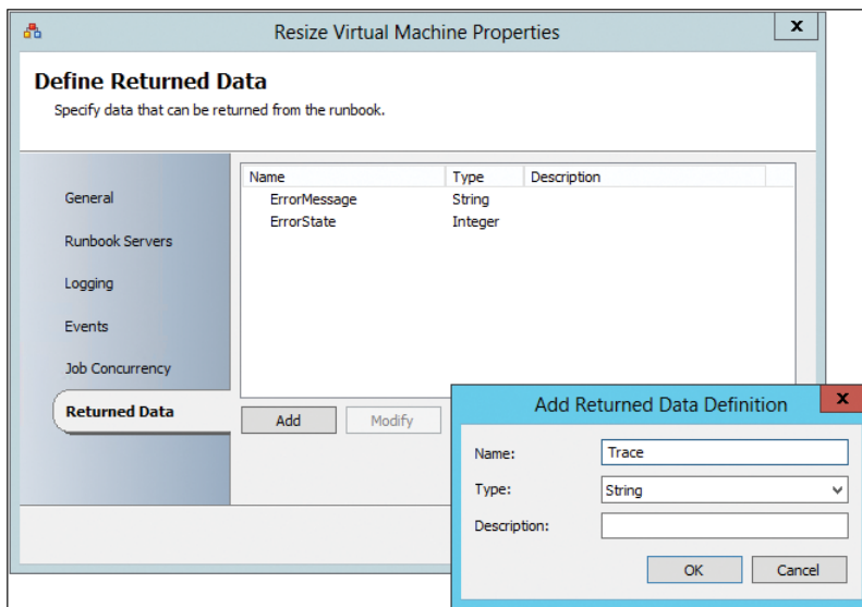
FIGURE 5-6 Setting up a runbook to publish data.
