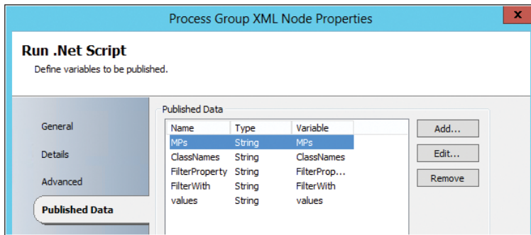
FIGURE 5-14 Published Data in the Run .Net Script activity.
