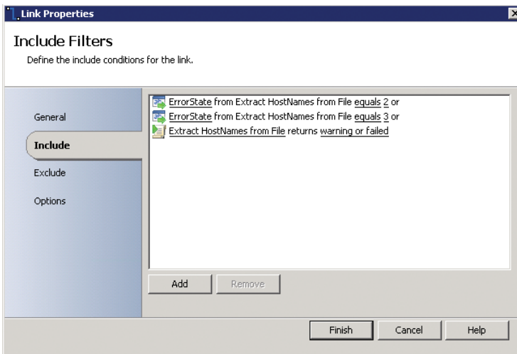
FIGURE 4-8 An example of error handling link properties.
