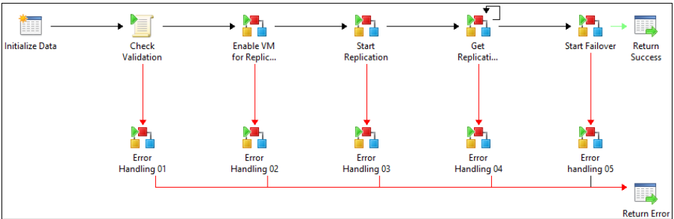
FIGURE 5-21 Validation inside of a control runbook.
