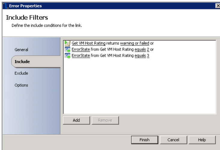
FIGURE 6-7 Include filters for the Return Error path.
