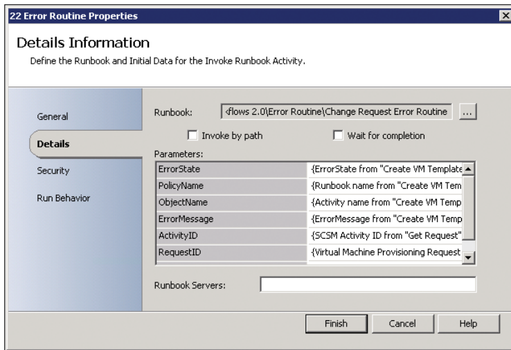
FIGURE 4-4 An example of an Orchestrator Return Data activity.
