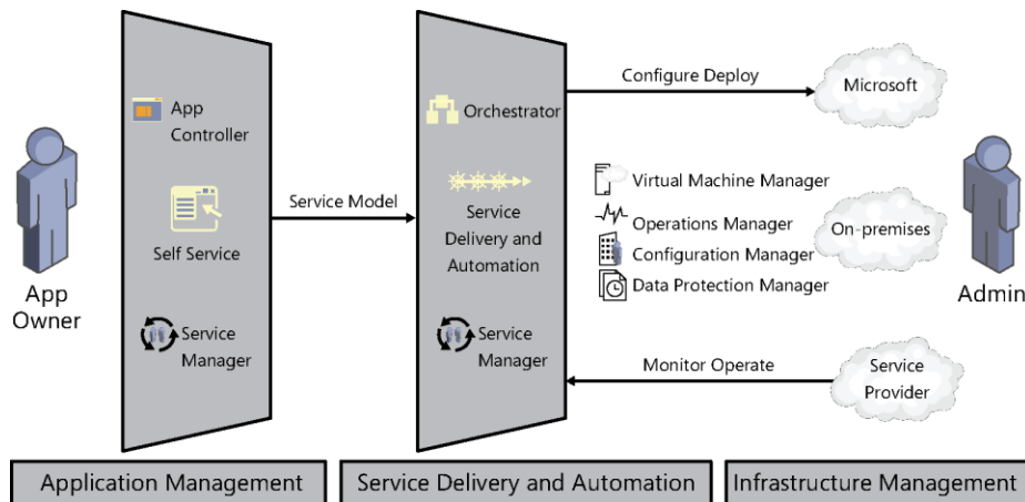
FIGURE 1-1 The System Center 2012 suite.
