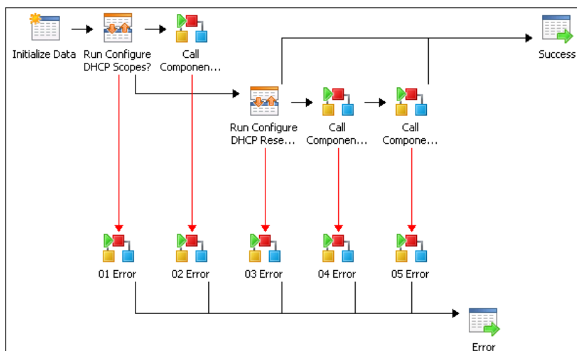
FIGURE 4-9 An example of an error handling design pattern.
