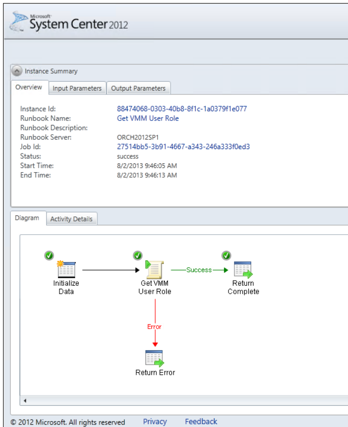
FIGURE 7-3 You can view the instance details of a runbook job.
