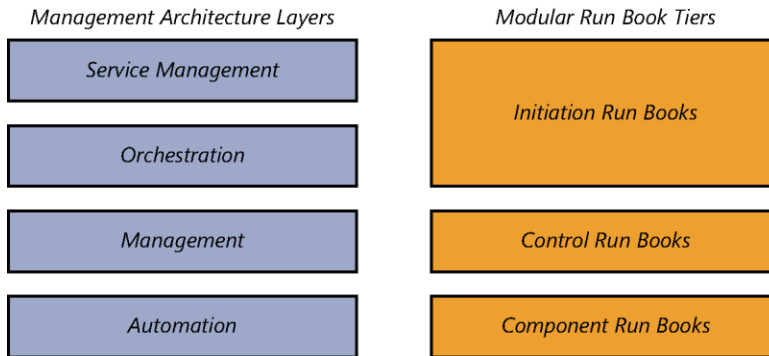
FIGURE 4-11 The layers of the modular runbook architecture.
