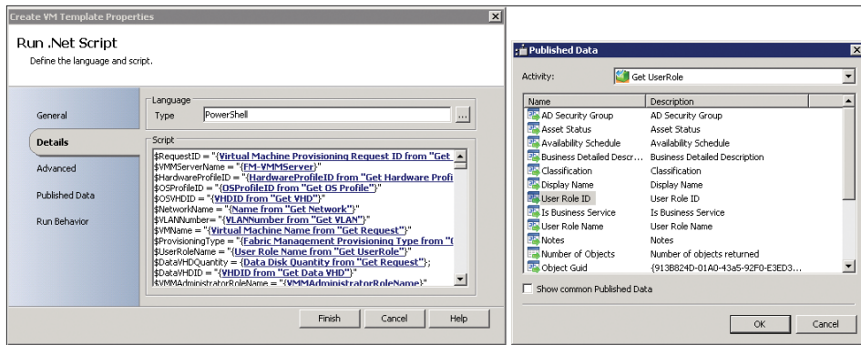
FIGURE 4-3 An example of the Orchestrator data bus.
