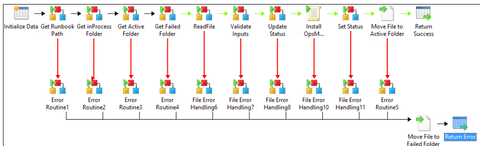
FIGURE 5-34 An example of a worker runbook.
