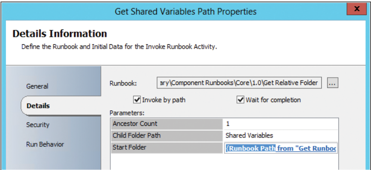
FIGURE 5-29 Setting the parameters for the Get Relative Folder runbook.
