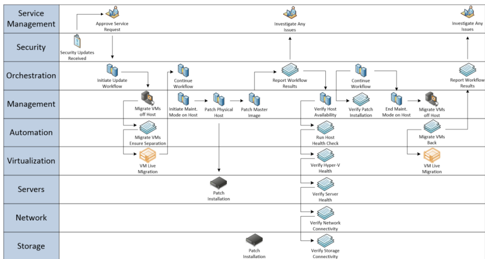
FIGURE 4-12 A sample process map.
