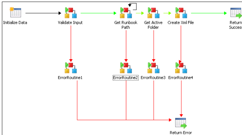
FIGURE 6-17 Initiation runbook for VM provisioning.
