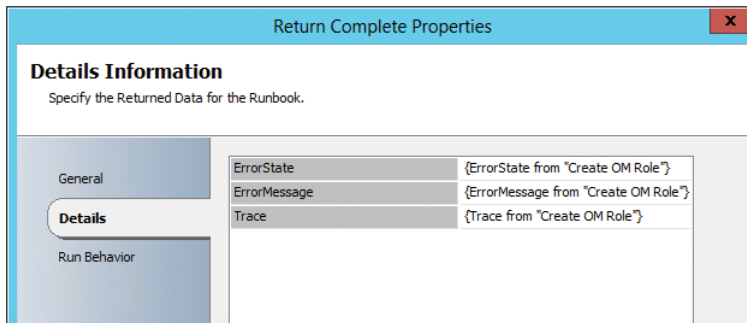
FIGURE 5-7 Setting up the Return Data activity.
