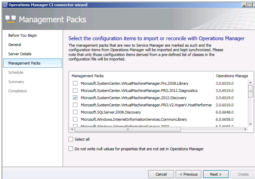
FIGURE B-6 The Management Pack page of the Operations Manager CI Connector Wizard.
