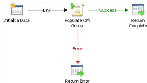
FIGURE 5-5 A sample runbook with color-coded links.
