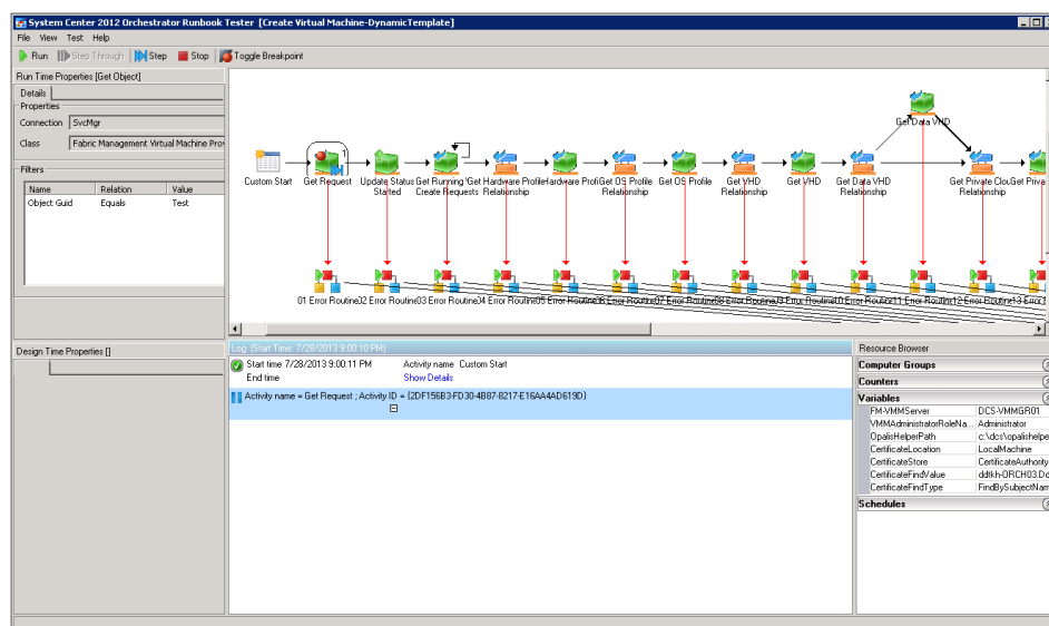
FIGURE 2-2 The Orchestrator Runbook Tester.
