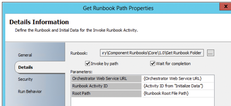
FIGURE 5-18 Setting the Invoke Runbook activity for component runbooks.
