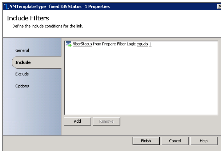
FIGURE 6-14 Filter logic for the VM Provisioning Engine runbook.
