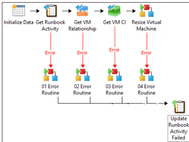
FIGURE 7-4 An example of a Service Manager initiation runbook.
