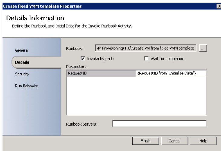
FIGURE 6-16 Invoke Runbook activity without waiting for completion.
