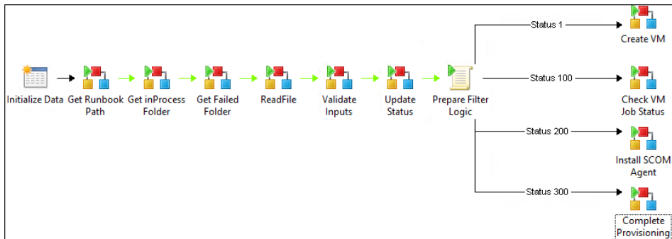
FIGURE 5-33 An engine runbook example.
