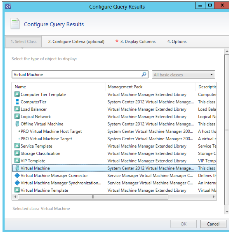
FIGURE 7-20 The Select Class tab in the Configure Query Results Wizard.
