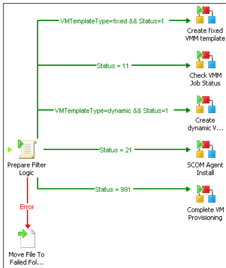
FIGURE 6-15 Link logic for the VM Provisioning Engine control runbook process flow.
