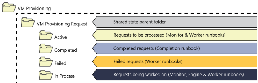
FIGURE 5-31 A Shared state folder example for VM provisioning.
