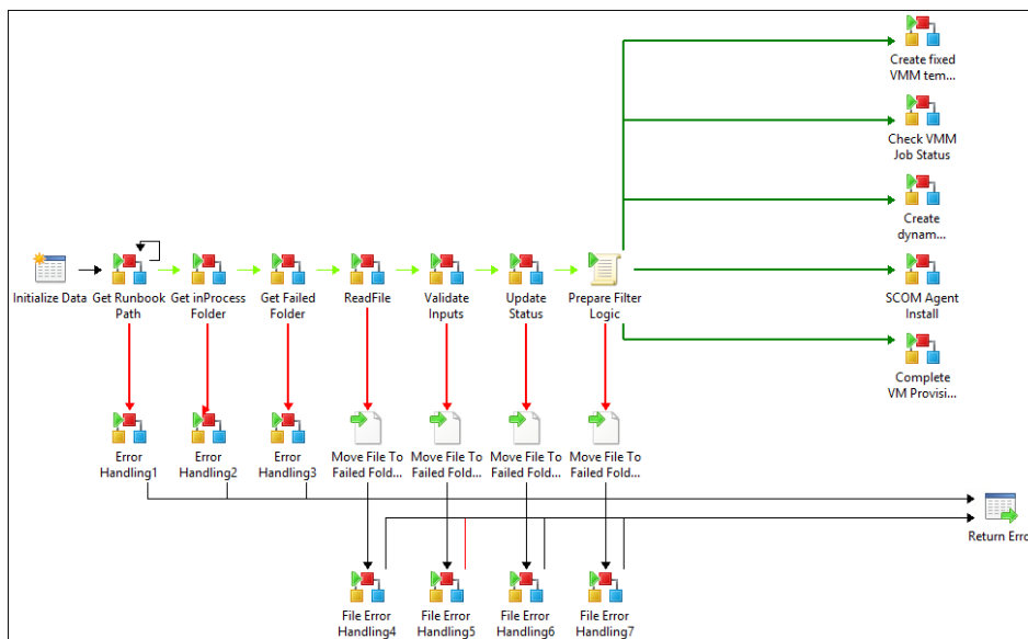
FIGURE 6-11 A diagram of the VM Provisioning Engine runbook.
