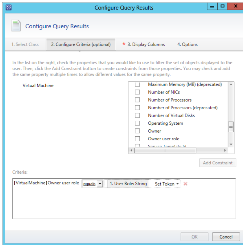
FIGURE 7-21 The Configure Criteria tab of the Configure Query Results Wizard.
