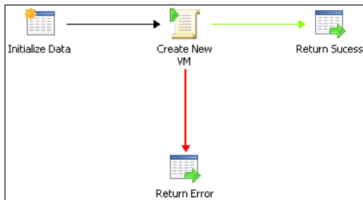
FIGURE 6-9 The CreateNewVM component runbook.
