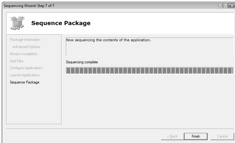
FIGURE 3-58 Sequencing progress.
