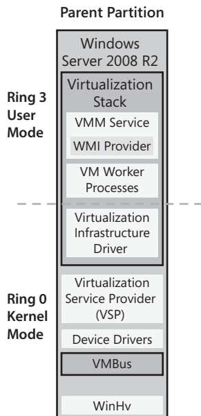
FIGURE 2-6 Detailed view of components of parent partition in Hyper-V.
