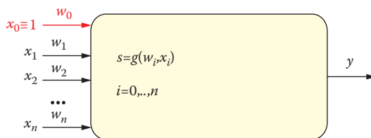
Figure 2.10 Application of bias parameter.
