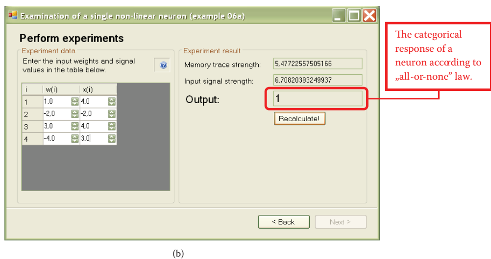
Figure 6.3 (continued) (a) Beginning of conversation with Example 06a program. (b) Next stage of conversation with Example 06a program.
