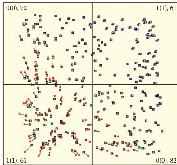
Figure 9.17 Slow and deliberate beginning of machine learning process in system with low value of learning coefficient (etha).
