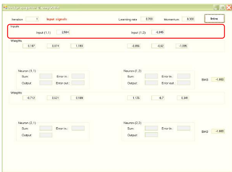
Figure 7.12 Appearance of input signals.
