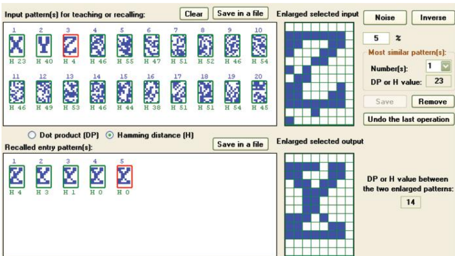
Figure 11.48 Overhearing observed for a minimally destroyed input signal if remembered patterns are not orthogonal.
