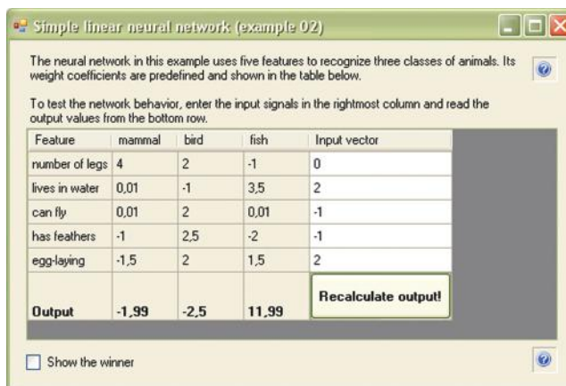
Figure 4.20 Program working to identify a fish.
