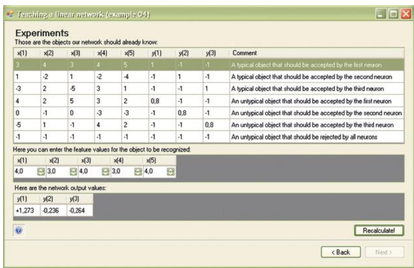
Figure 5.10 Characteristics of network examination in Example 04 program.
