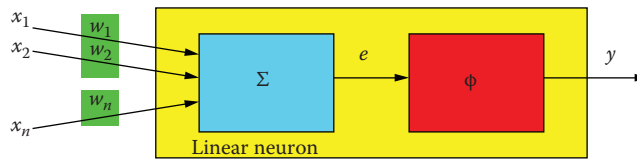
Figure 2.13 Structure of a neuron as a processor—the basis for building neural networks.
