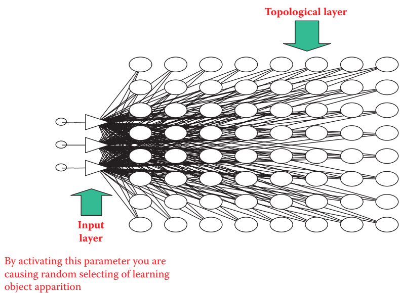
Figure 10.3 Structure of self-organizing neural network.
