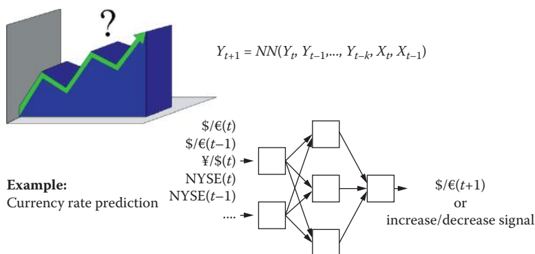
Figure 2.36 Currency rate estimation using a neural network.
