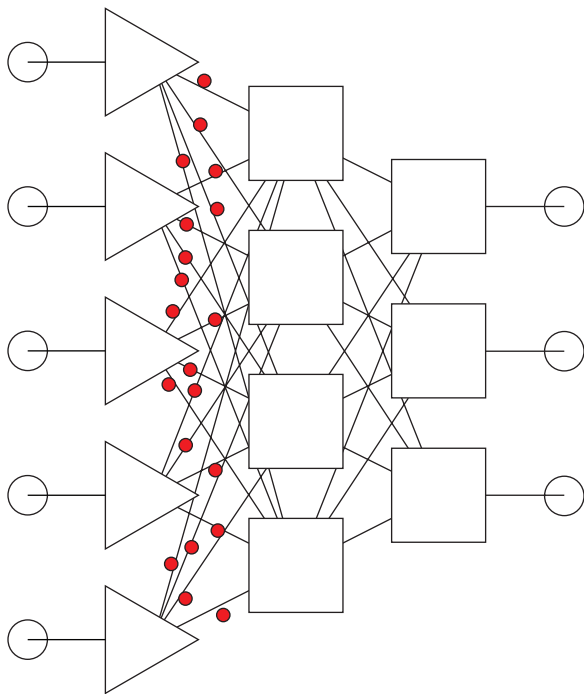
Figure 2.19 Unprocessed input signals are sent to all neurons in a hidden layer.
