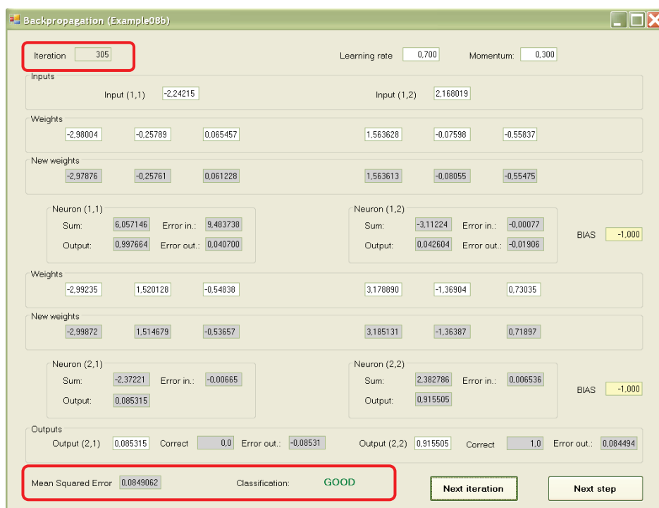
Figure 7.20 Final result of teaching.
