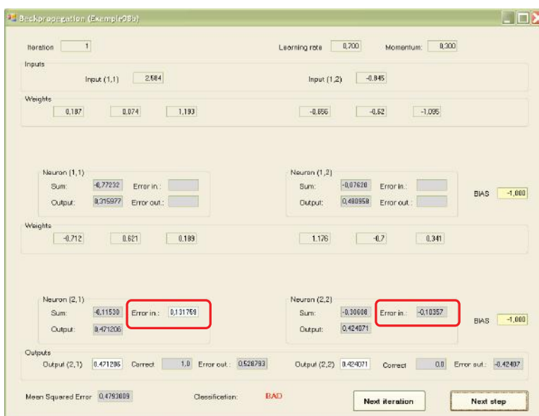
Figure 7.17 Transfer of errors on inputs of neurons.
