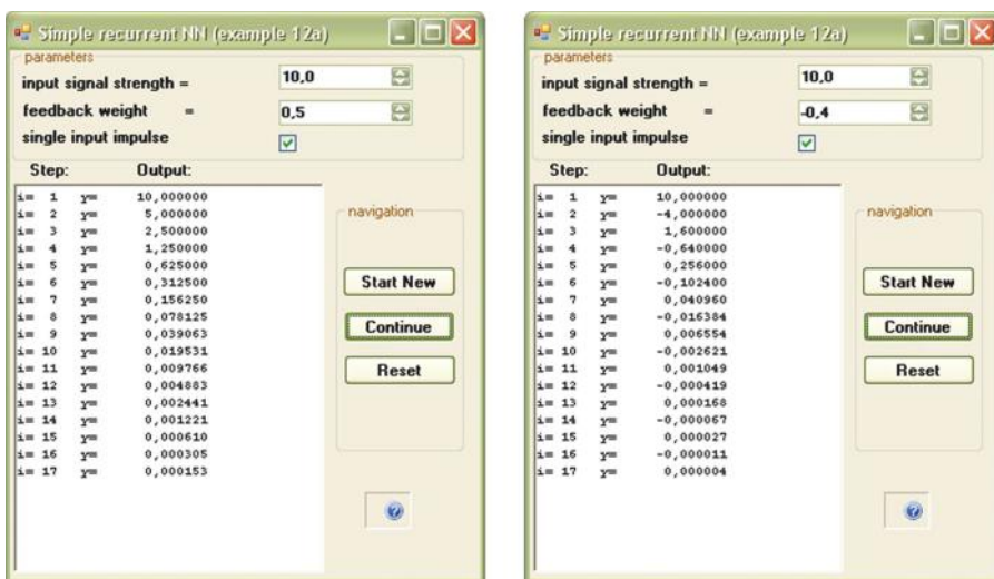
Figure 11.7 Stable progress of system with feedback after decreasing value of weight factor well below stabilization point.
