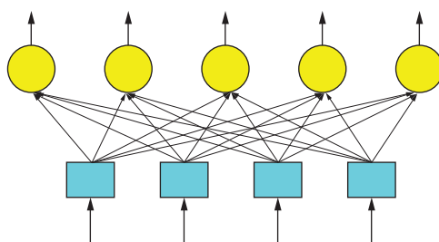
Figure 2.38 Single-layered network.
