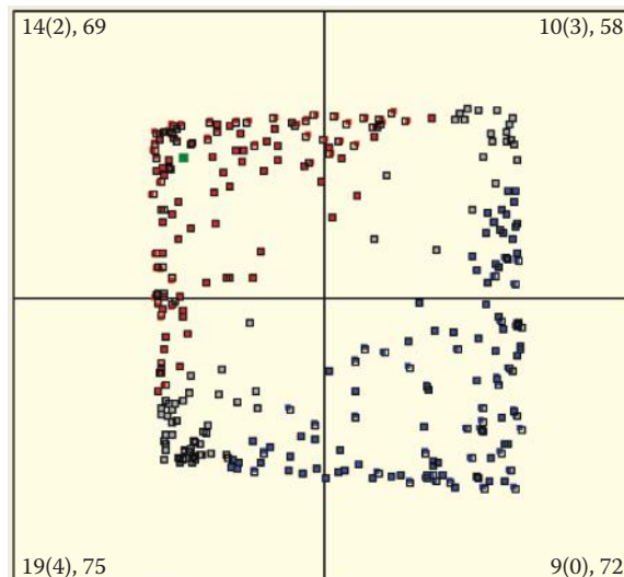
Figure 9.18 Similar stage of machine learning process shown in Figure 9.14. We see numerous “vacant” neurons with low values of learning coefficients.
