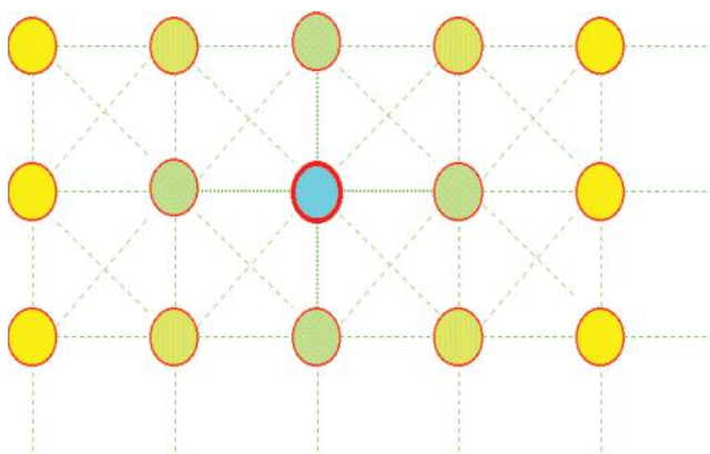
Figure 10.10 Richer neighborhood.
