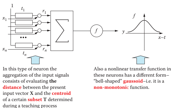
Figure 2.15 Structure and peculiar properties of radial neuron.
