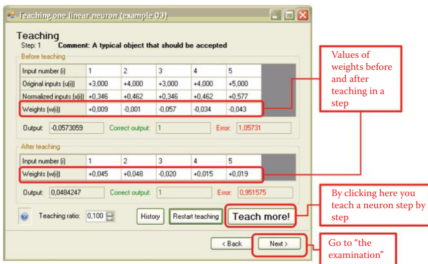
Figure 5.2 Beginning of teaching a neuron.
