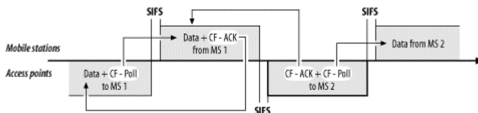
Figure 8-6. CF-Ack+CF-Poll usage
