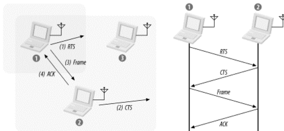
Figure 3-3. RTS/CTS clearing
