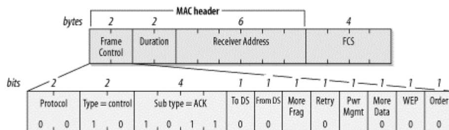
Figure 4-17. ACK frame
