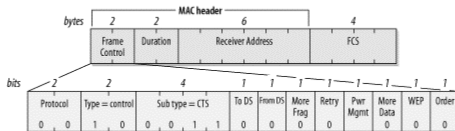
Figure 4-15. CTS frame
