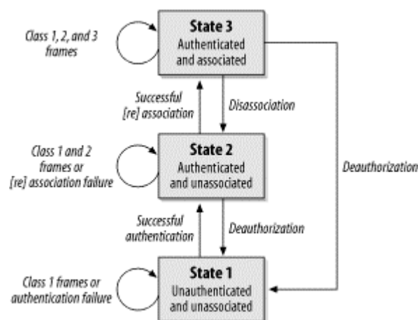
Figure 4-48. Overall 802.11 state diagram
