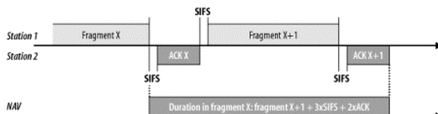
Figure 4-3. Duration settings on nonfinal fragment
