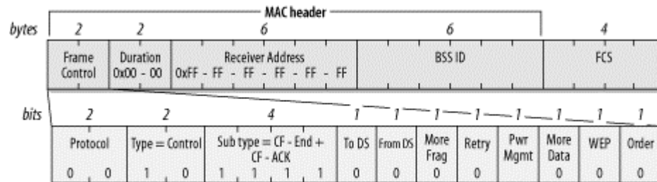
Figure 8-8. CF-End+CF-Ack frame
