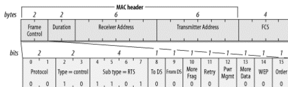
Figure 4-13. RTS frame
