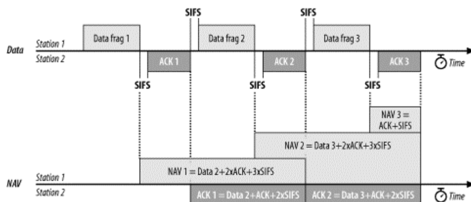
Figure 3-16. Fragmentation
