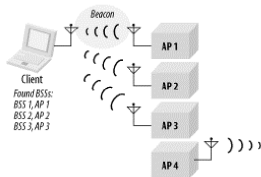
Figure 7-2. Passive scanning
