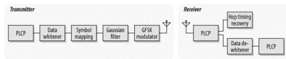
Figure 10-10. Frequency-hopping transceiver
