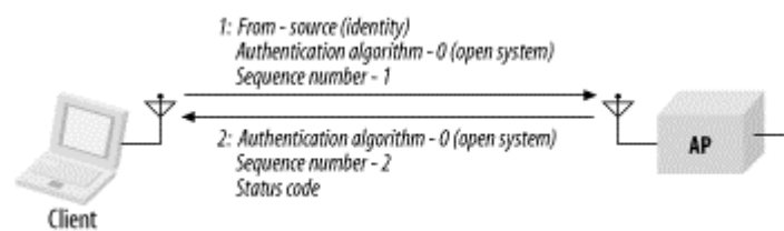
Figure 7-4. Open-system authentication exchange
