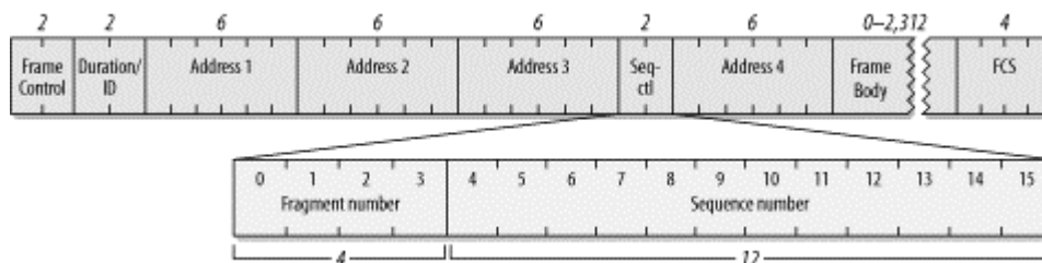
Figure 3-12. Sequence Control field
