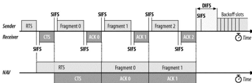
Figure 3-8. Fragmentation burst
