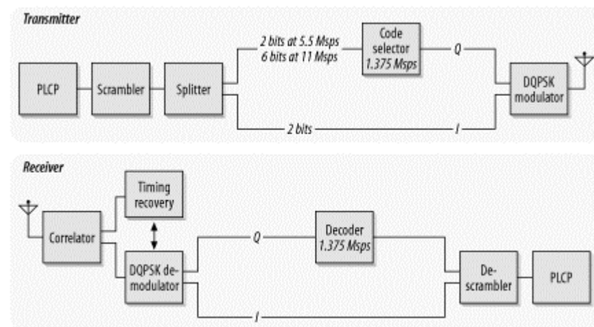
Figure 10-28. HR/DSSS transceiver
