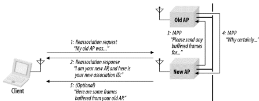
Figure 7-8. Reassociation procedure
