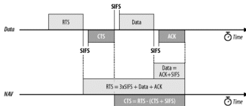
Figure 3-17. RTS/CTS lockout
