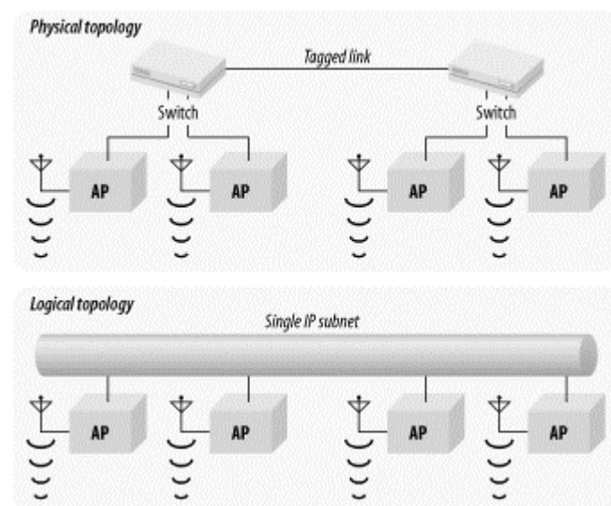
Figure 15-3. Using VLANs to span multiple switches
