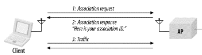
Figure 7-7. Association procedure
