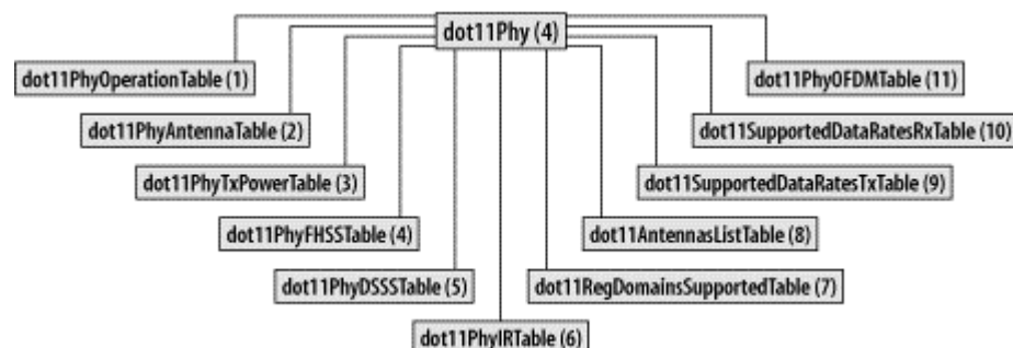
Figure A-7. Physical-layer MIB branches
