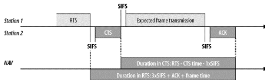
Figure 4-16. CTS duration
