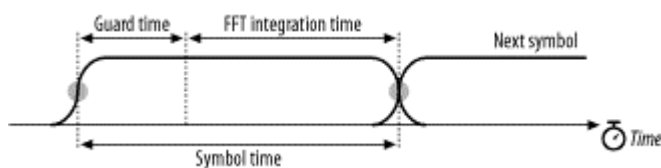
Figure 11-7. Cosine windowing technique
