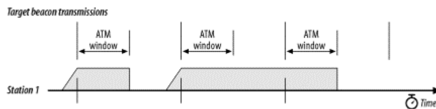
Figure 7-15. ATIM effects on power-saving modes
