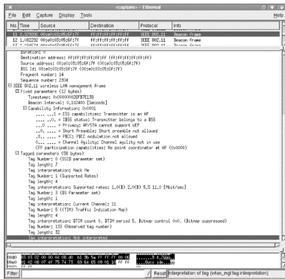
Figure 16-6. Beacon frame decode
