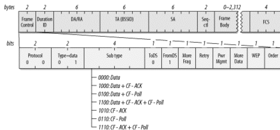
Figure 4-9. Data frames from the AP
