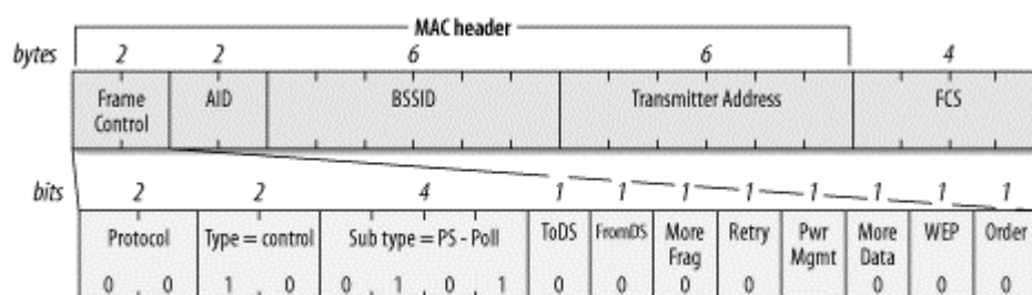
Figure 4-19. PS-Poll frame
