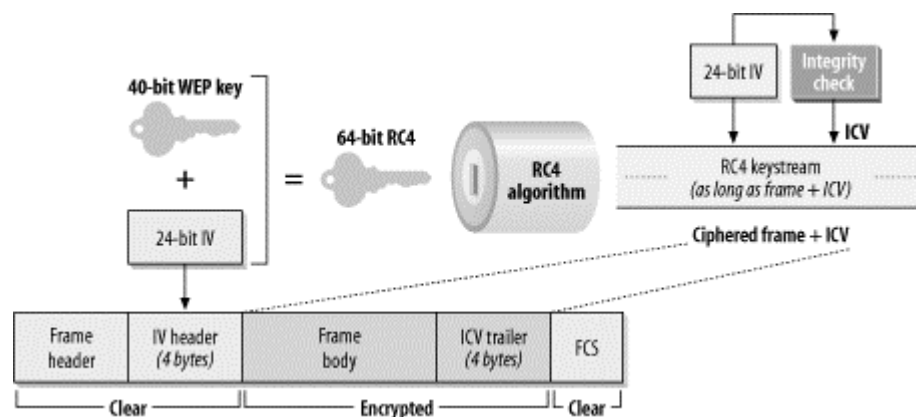
Figure 5-3. WEP operations
