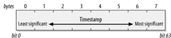
Figure 4-28. Timestamp field
