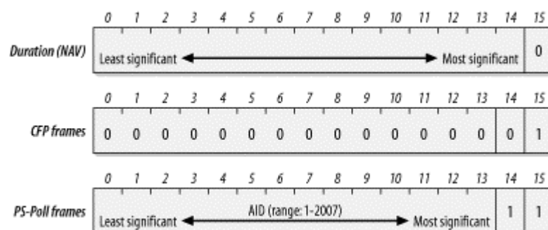
Figure 3-11. Duration/ID field
