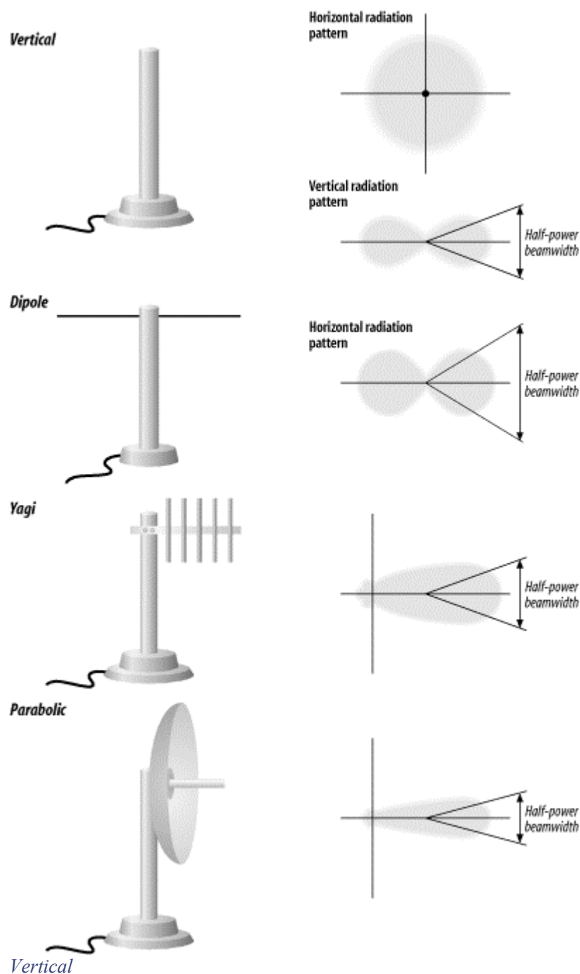
Figure 15-5. Antenna types
