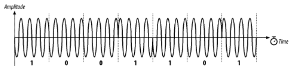
Figure 10-20. The letter M encoded in DBPSK
