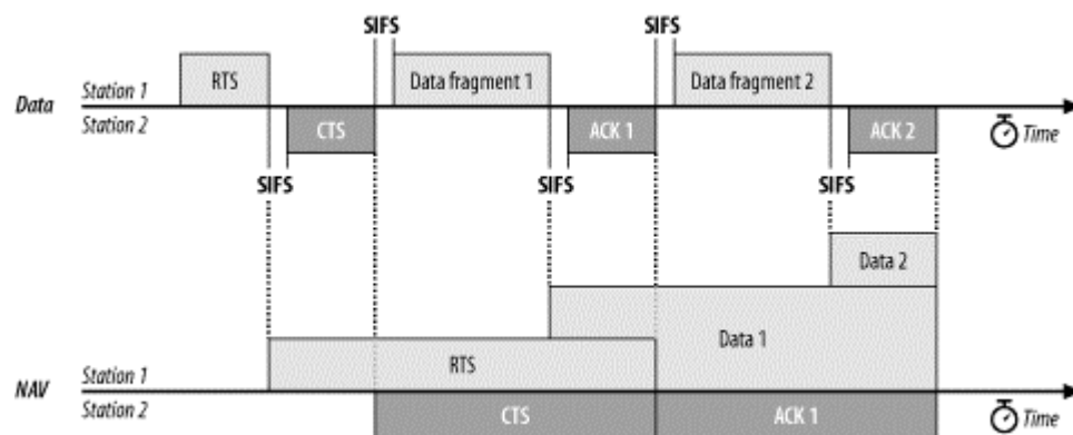
Figure 3-18. RTS/CTS with fragmentation
