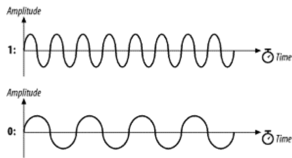
Figure 10-5. 2-level GFSK
