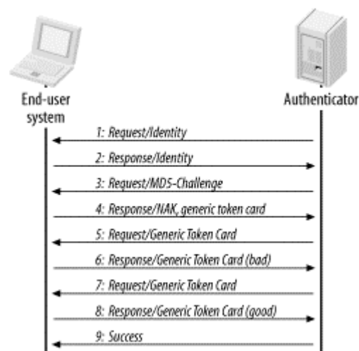
Figure 6-5. Sample EAP exchange
