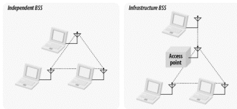
Figure 2-4. Independent and infrastructure BSSs
