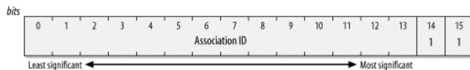
Figure 4-27. Association ID field
