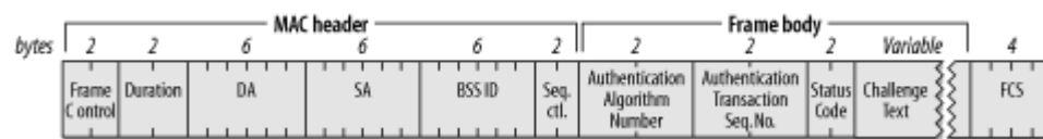
Figure 4-47. Authentication frames
