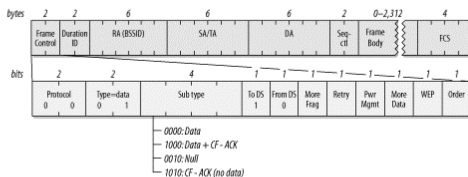
Figure 4-10. Data frames to the AP
