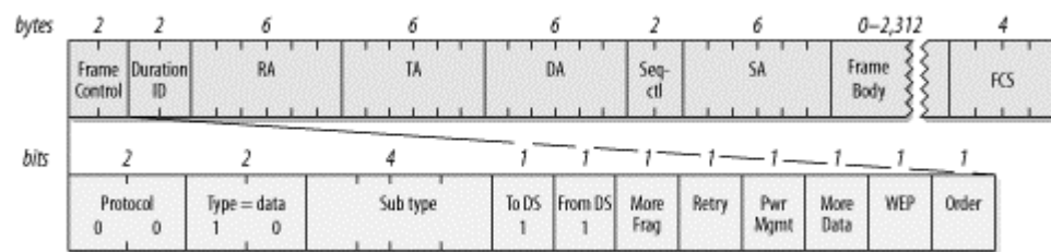
Figure 4-11. WDS frames
