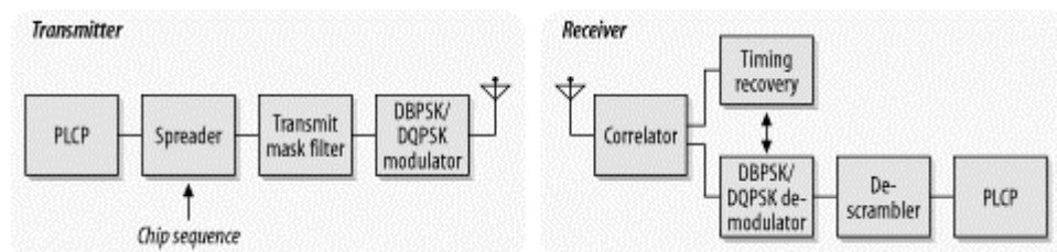
Figure 10-24. Direct-sequence transceiver
