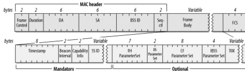
Figure 4-39. Beacon frame
