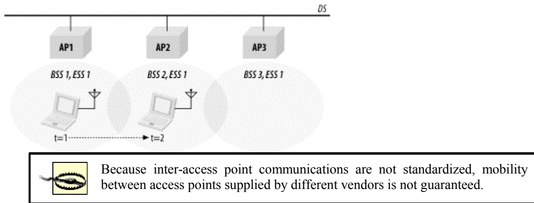
Figure 2-9. BSS transition
