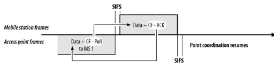
Figure 8-3. Data+CF-Ack usage
