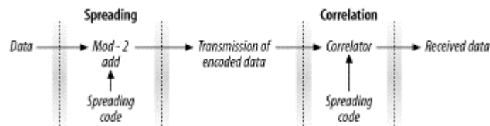
Figure 10-13. Chipping
