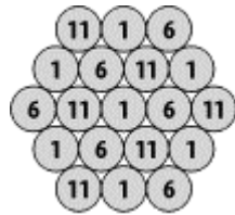
Figure 15-6. Frequency planning
