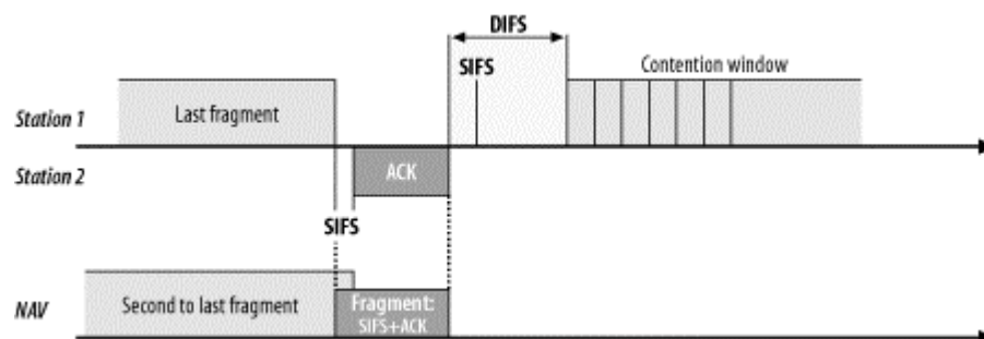
Figure 4-2. Duration setting on final fragment
