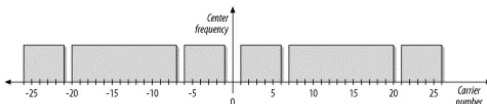
Figure 11-8. Structure of an OFDM channel
